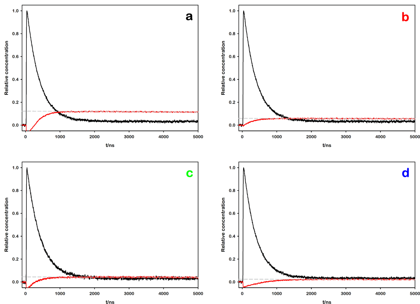
Figure 5. Transient absorption kinetic traces of the photoexcited samples (Ru–MV 2+ in 0.1 mM NaOH, pH = 10.00) after laser flash photolysis ( \lambda_{\text{exc}} = 355 nm). The black lines show the decay of the ^*\text{[Ru(bpy)}_3\text{]}^{2+} at 450 nm, used as transient actinometer. The red lines display the growth of MV •+ for (a) [\text{Ru(bpy)}_3]^{2+} , (b) [\text{Ru(bpy)}_2(\text{dcbpy})]^+ , (c) [\text{Ru(bpy)}(\text{dcbpy})_2]^{2-} , and (d) [\text{Ru(dcbpy)}_3]^{4-} as the photosensitizer. The gray dashed lines represent the linear fittings of the 605 nm kinetic traces, used to extrapolate relative MV •+ concentration at t = 0 .
