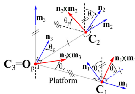
Figure 5. Geometric relationships among the unit vectors \mathbf{n}_i , \mathbf{m}_i , and \mathbf{n}_i \times \mathbf{m}_i , for i = 1, 2, 3 , in the platform of the 3-XXRRU shown in Figure 4.
