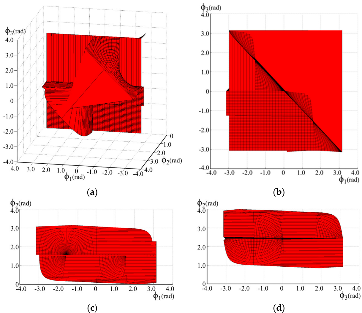
Figure 6. Computed free-from-singularity orientation workspace (the parameters \phi_1 , \phi_2 , and \phi_3 on the axes are the ZYZ Euler angles that locate the orientation of O_px_py_pz_p with respect to O_0x_0y_0z_0 ): (a) 3D view, (b) projection onto the \phi_1\phi_3 -plane, (c) projection onto the \phi_1\phi_2 -plane, and (d) projection onto the \phi_2\phi_3 -plane.
