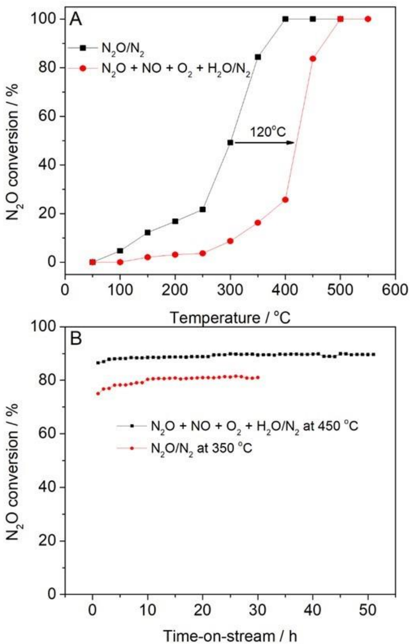
Figure 7. The catalytic activity of CeCoAl catalyst: A) Comparison of absence and presence of inhibitors and B) Stability test in absence and presence of inhibitors. Reaction conditions: 0.3 g catalyst, 80 mL min -1 of 1000 ppm N 2 O/N 2 (absence of inhibitors) or 1000 ppm N 2 O + 200 ppm NO + 20,000 ppm O 2 + 2500 ppm H 2 O/N 2 (presence of inhibitors).
