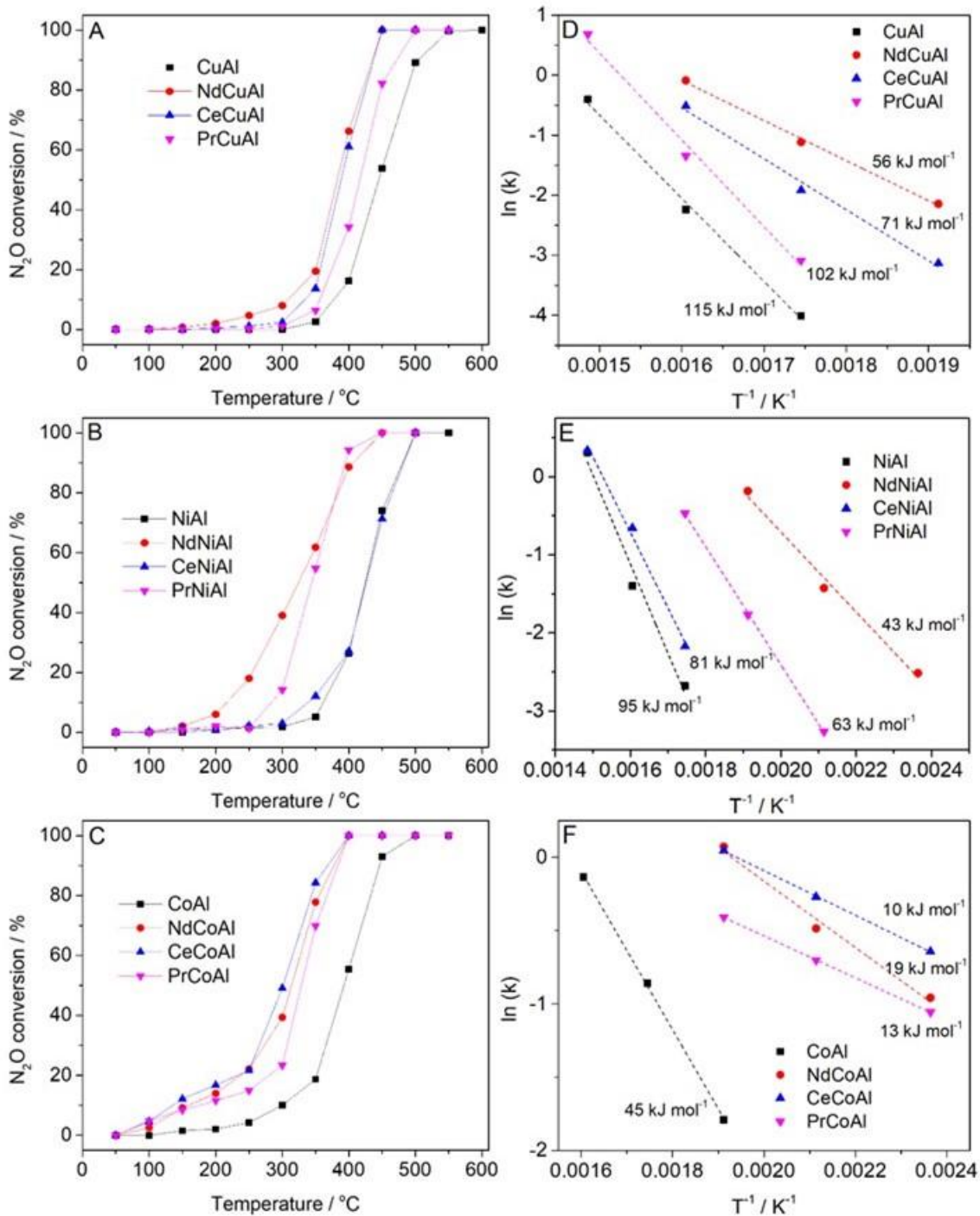
Figure 6. N 2 O conversion (A, B, C) and Arrhenius plots for calculation of apparent activation energies (D, E, F) of different RMAI mixed metal oxides (R = Nd, Ce, Pr and M = Cu, Ni, Co). Reaction conditions: 0.3 g catalyst, 80 mL min -1 of 1000 ppm N 2 O/N 2 . To minimize the influence of heat generated from the exothermic reaction, E a calculations were performed for data points with conversion lower than 30%.
