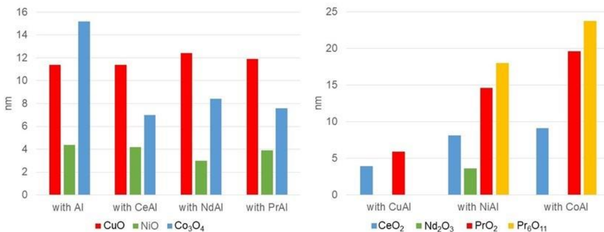
Figure 2. Evolution of the Scherrer crystallite sites of (A) transition metal oxides in the presence of different REE and (B) rare earth oxides in the presence of different transition metals.
