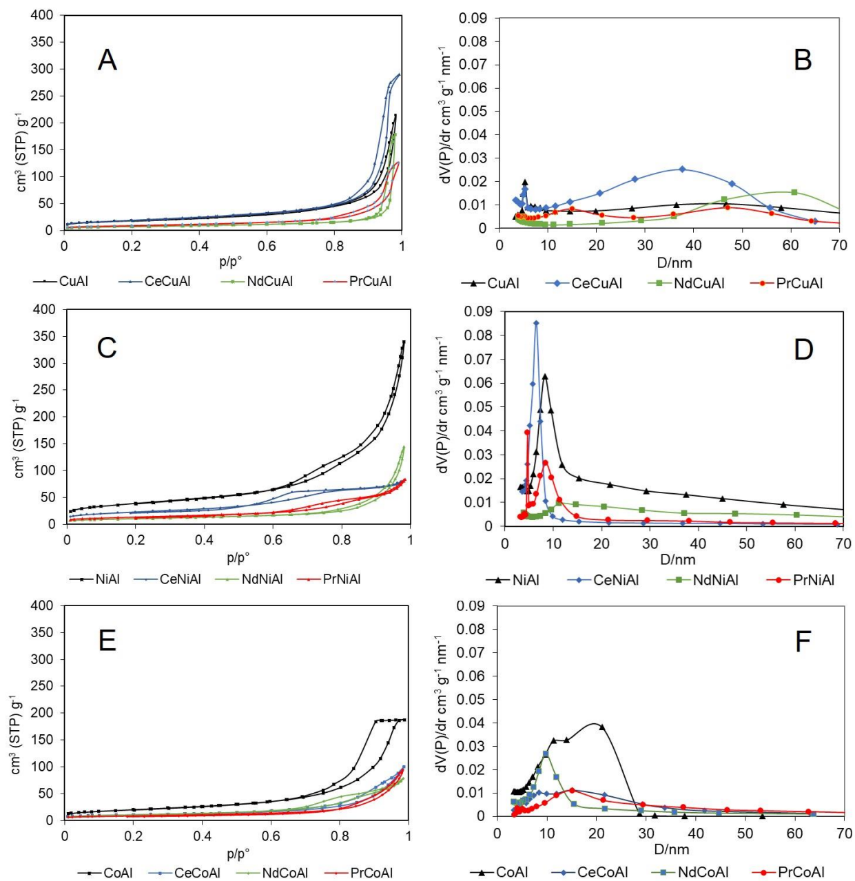
Figure 3. N 2 adsorption-desorption isotherms and mesopore distributions (from the desorption branch of the isotherms) of catalysts, respectively, the copper (A, B), nickel (C, D), and cobalt-containing catalysts (E, F).
