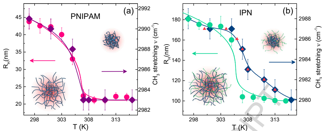
Figure 5: Hydrodynamic radius R_H and \text{CH}_3 frequency as a function of temperature for (a) PNIPAM and (b) IPN microgels at low concentrations. (b) Comparison of the \text{CH}_3 frequency behaviour for IPN microgels at C_w=0.1\% (red triangles) and C_w=0.3\% (blue diamonds). Magenta and green solid lines are the fit of R_H(T) through the Flory-Rehner theory, purple and blue solid lines are guide to eyes for the \text{CH}_3 frequency behaviour.
