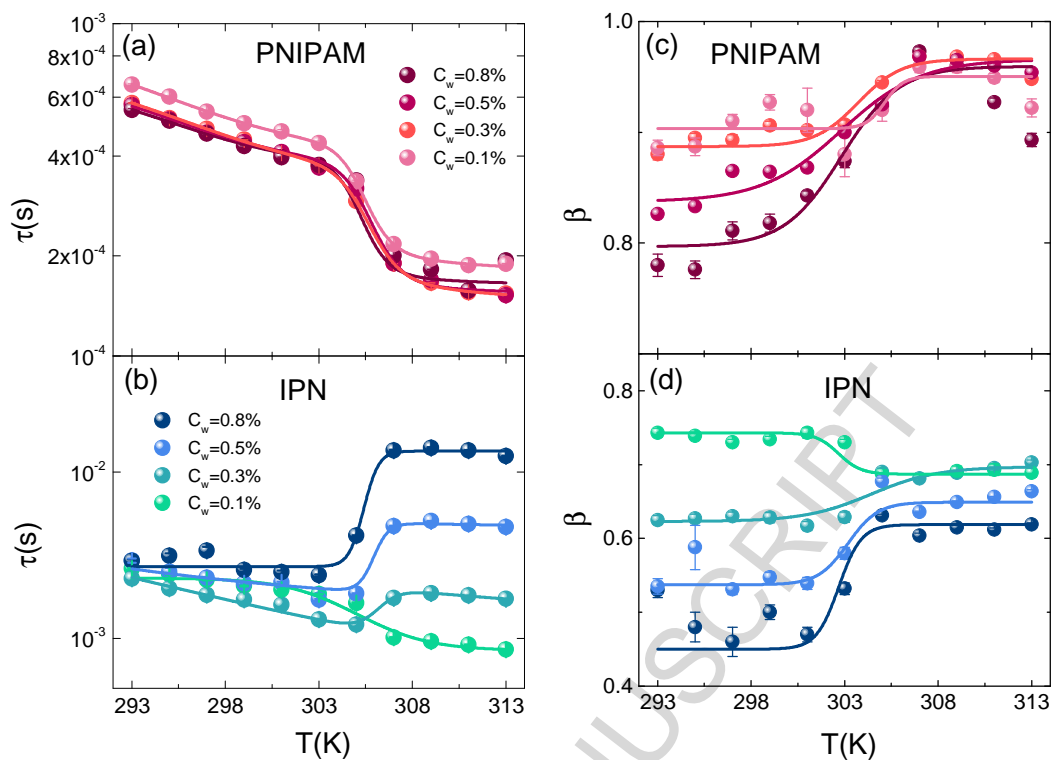
Figure 2: (a,b) Relaxation time and (c,d) shape parameter as a function of temperature for PNIPAM and IPN microgels at C_{PAAc} = 19.2\% at the indicated weight concentrations. Solid lines are guides to eyes.
