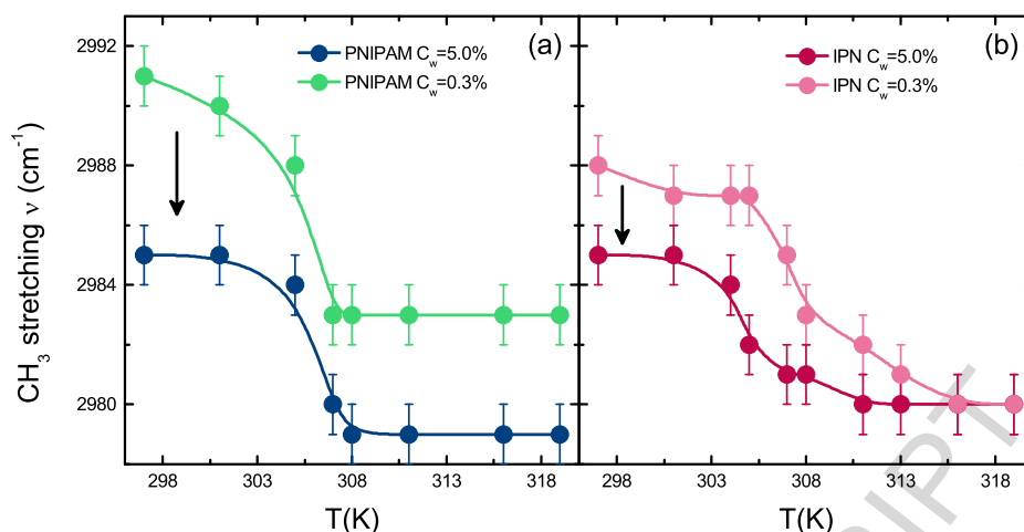
Figure 6: CH 3 frequency as a function of temperature for (a) PNIPAM and (b) IPN microgels at C_w = 0.3\% and C_w = 5.0\% . Solid lines are guides to eyes. The arrows underline the reduction of CH 3 frequency on increasing microgel concentration.
