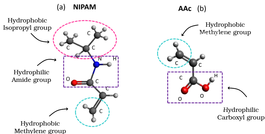
Figure 1: Sketch of (a) NIPAM and (b) AAc molecular structure.
