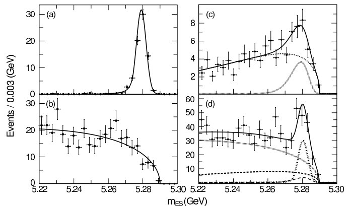
FIG. 2: Fits to the M(X_s) = 1.4 - 1.5 GeV bin for (a) correctly reconstructed signal Monte Carlo events; (b) simulated continuum background; (c) simulated cross-feed and hadronic B decay backgrounds, where the contributions from the peaking (dotted) and combinatorial (dashed) backgrounds are shown separately; (d) on-peak data, where the contributions from the signal (dotted-dashed), continuum background (dotted), peaking B background (long-dashed), and combinatorial B background (dashed) are shown separately.
