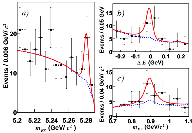
FIG. 2: Distributions of the fit variables in K^* \ell^+ \ell^- data (points), compared with projections of the simultaneous fit (curves): (a) m_{ES} after requiring -0.11 < \Delta E < 0.05 GeV and 0.817 < m_{K\pi} < 0.967 GeV/ c^2 , (b) \Delta E after requiring |m_{ES} - m_B| < 6.6 MeV/ c^2 ( 2.6\sigma ), 0.817 < m_{K\pi} < 0.967 GeV/ c^2 , and (c) m_{K\pi} after requiring |m_{ES} - m_B| < 6.6 MeV/ c^2 and -0.11 < \Delta E < 0.05 GeV. The solid curve is the sum of all fit components, including signal; the dashed curve is the sum of all background components.
