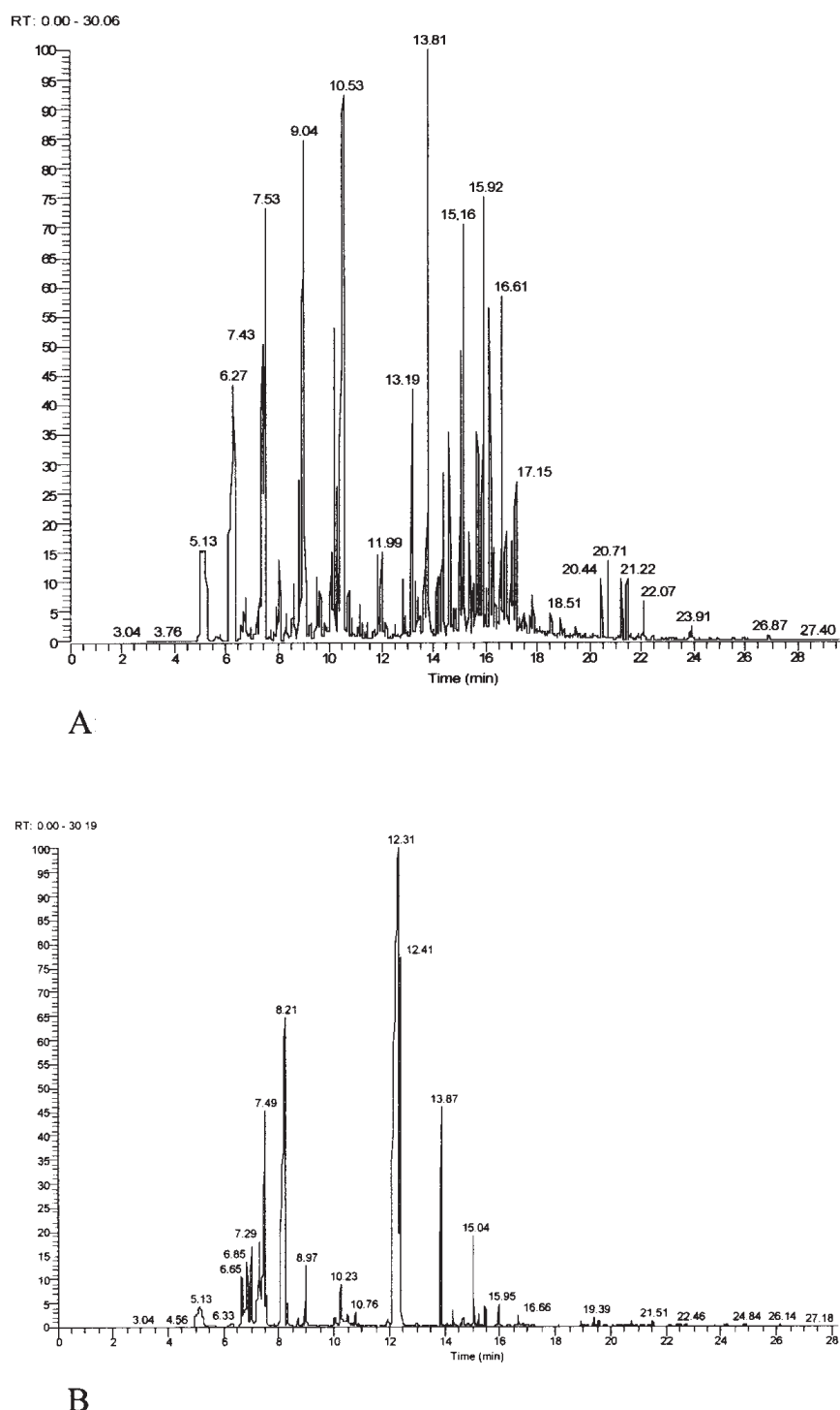
Figure 2. Chromatograms obtained with GC/MS of Satureja montana (A) and Satureja hortensis (B) essential oils.
