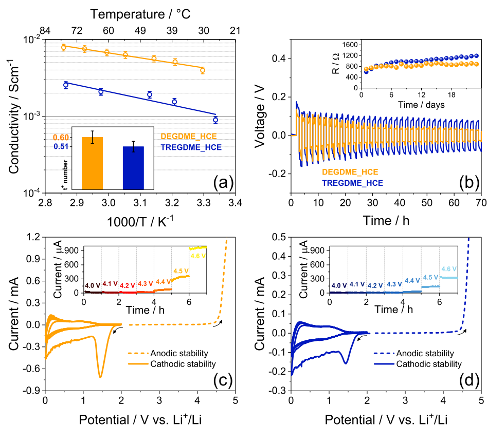
Figure 4. (a) Arrhenius conductivity plots and Li + transference number values (inset, see the determination method in the Experimental Section ) of DEGDME_HCE (orange) and TREGDME_HCE (blue). (b) Lithium stripping/deposition tests performed on Li/electrolyte/Li symmetrical cells employing either DEGDME_HCE (orange) or TREGDME_HCE (blue) by applying a current of 0.1 mA cm -2 ; inset shows the interphase resistance trends recorded upon Li/electrolyte/Li symmetrical cells aging employing DEGDME_HCE (orange) or TREGDME_HCE (blue) through EIS in the 500 kHz to 100 mHz frequency range by applying a signal of 10 mV (see the corresponding Nyquist plots in Figure S3 and the related NLLS analyses in Tables S1 and S2 in the Supporting Information ). (c,d) Electrochemical stability window determined by means of CV in the cathodic region (solid line) and LSV in the anodic one (dashed line) performed on lithium cells employing either (c) DEGDME_HCE or (d) TREGDME_HCE, and SPC as the working electrode; scan rate: 0.1 mV s -1 , CV potential range: 0.01–2 V vs Li + /Li; insets show the chronoamperometry test carried out in the 4.0–4.6 V vs Li + /Li potential range through voltage increase by steps of 0.1 V every hour.
