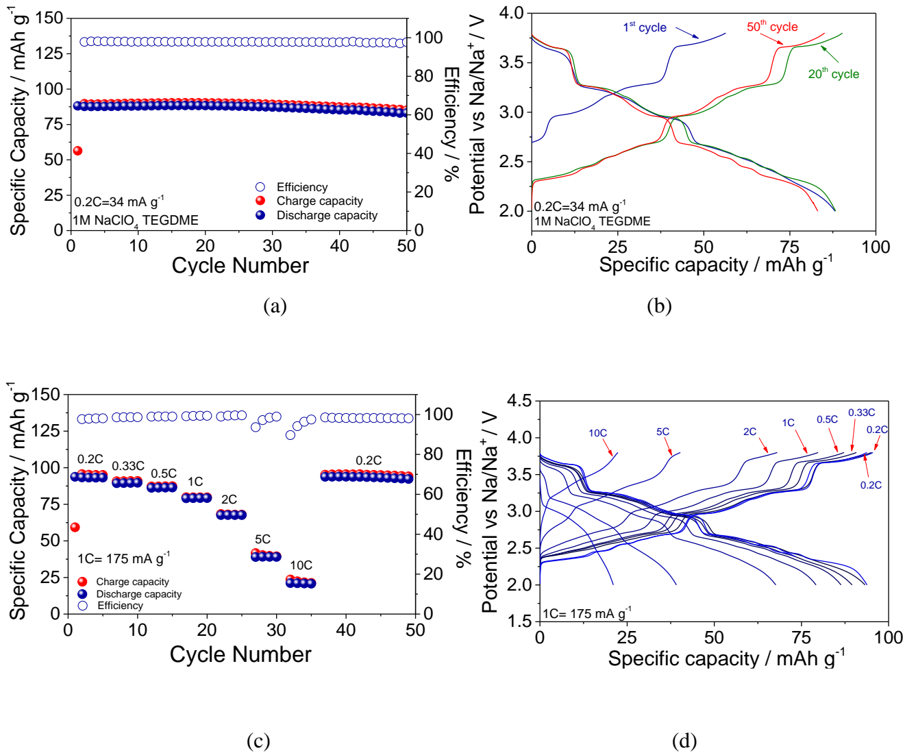
Figure S1. (a) Galvanostatic cycling behavior and (b) corresponding voltage profile of the Na/1M NaClO 4 -TEGDME/Na 0.7 CoO 2 half-cell studied at 34 mA g -1 current within the 2.0-3.8 V (vs Na/Na + ) voltage range. (c) Cycling trend at increasing current densities and (d) corresponding voltage curves of the Na/1M NaClO 4 -TEGDME/Na 0.7 CoO 2 half-cell.
