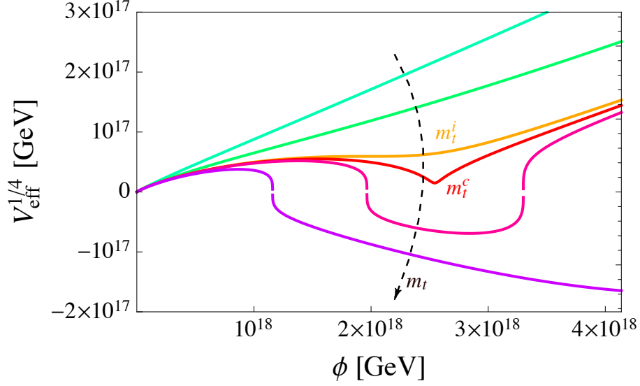
Figure 1: Sketch of the shape of SM effective potential at high energy in the Landau gauge, for increasing values of the top mass from top to bottom. Two peculiar stationary configuration can be identified: two degenerate vacua and a rising point of inflection, associated respectively to m_t^c and m_t^i .
