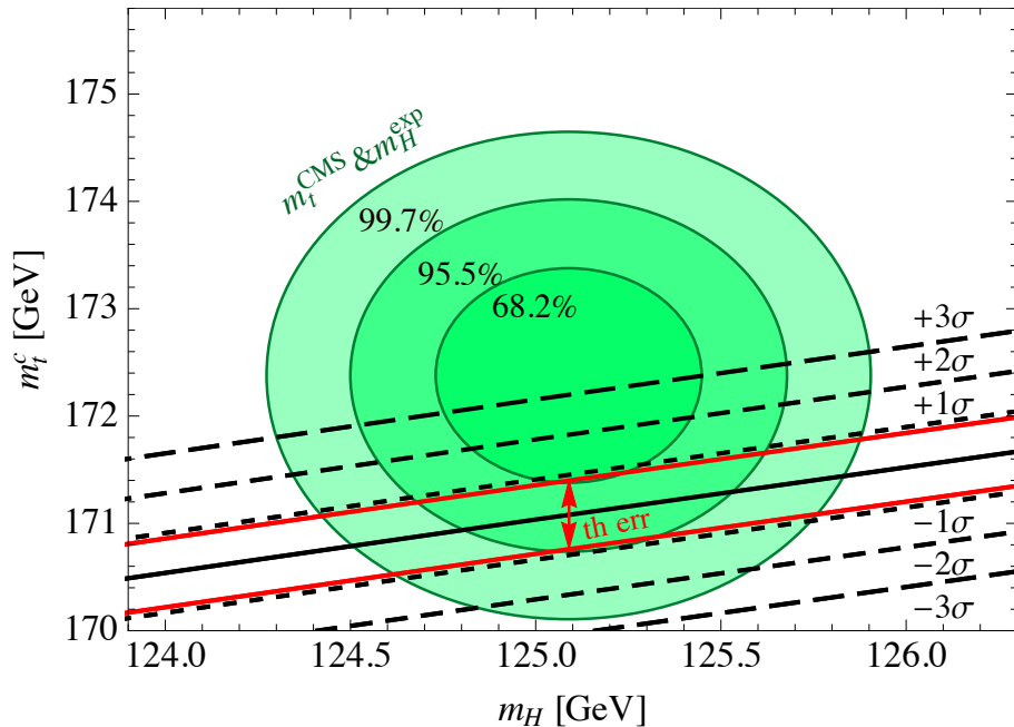
Figure 4: Lines for which the Higgs potential develops a second degenerate minimum at high energy. The solid line corresponds to the central value of \alpha_s^{(5)} ; the dashed lines are obtained by varying \alpha_s^{(5)} in its experimental range, up to 3\sigma . The (red) arrow represents the theoretical error in the position of the lines. The (green) shaded regions are the covariance ellipses obtained combining m_t^{\text{CMS}} = 172.38 \pm 0.66 GeV [49] and m_H^{\text{exp}} = 125.09 \pm 0.24 GeV.
