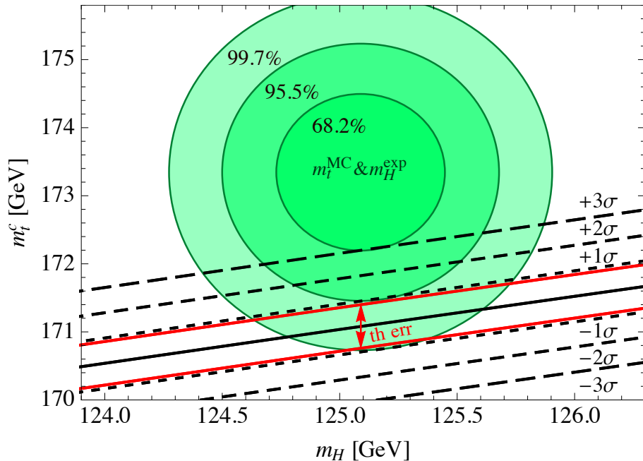
Figure 2: Lines for which the Higgs potential develops a second degenerate minimum at high energy. The solid line corresponds to the central value of \alpha_s^{(5)} ; the dashed lines are obtained by varying \alpha_s^{(5)} in its experimental range, up to 3\sigma . The (red) arrow represents the theoretical error in the position of the lines. The (green) shaded regions are the covariance ellipses obtained combining m_t^{MC} = 173.34 \pm 0.76 GeV and m_H^{exp} = 125.09 \pm 0.24 GeV; the probability of finding m_t^{MC} and m_H inside the inner (central, outer) ellipse is equal to 68.2% (95.5%, 99.7%).
