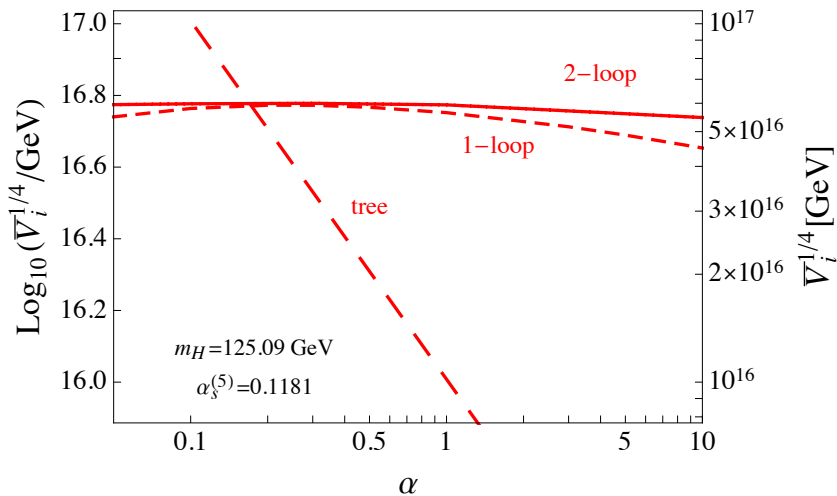
Figure 6: Dependence of \bar{V}_i^{-1/4} on \alpha . For definiteness, \alpha_s^{(5)} and m_H are assigned to their central values.
