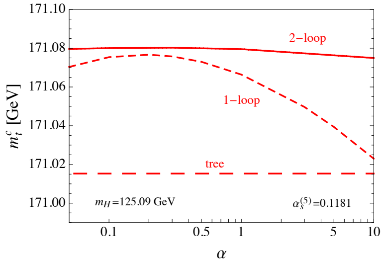
Figure 3: Dependence of m_t^c on \alpha , for increasing level of the effective potential expansion. We choose the central values for m_H and \alpha_s^{(5)} .
