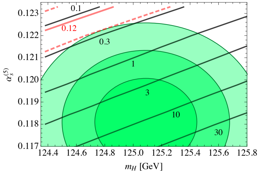
Figure 7: Contour levels of r in the plane (m_H, \alpha_s^{(5)}) . The theoretical uncertainty corresponding to r = 0.12 is shown by means of the (red) dashed lines. The shaded regions are the covariance ellipses indicating that the probability of finding the experimental values of m_H and \alpha_s^{(5)} inside the ellipses are respectively 68.2%, 95.4%, 99.7%.
