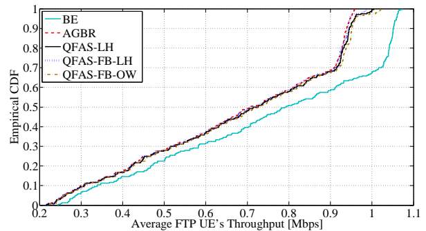
Fig. 8. Empirical CDF of the Average FTP UE's throughput.
