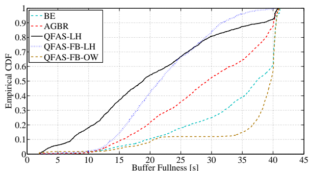
Fig. 5. Empirical CDF of the buffer fullness evaluated at each chunk request of the clients
