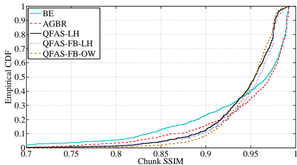
Fig. 3. Empirical CDF of the chunk-by-chunk SSIM at the clients
