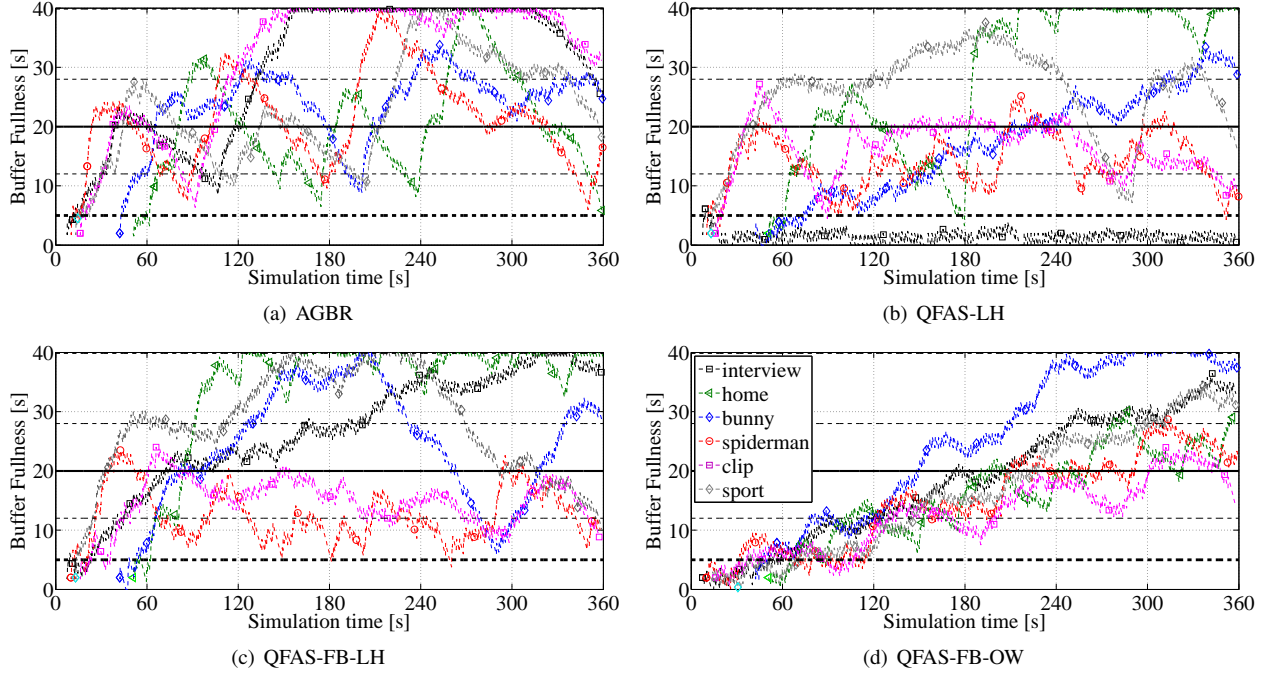
Fig. 7. An example (one drop of simulation) of the evolution of the buffer fullness at the clients for the GBR-aware strategies.
