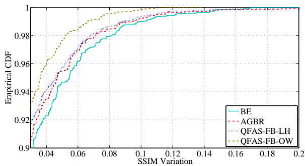
Fig. 4. Empirical CDF of the chunk-by-chunk SSIM variation \delta_{\text{SSIM}} at the clients
