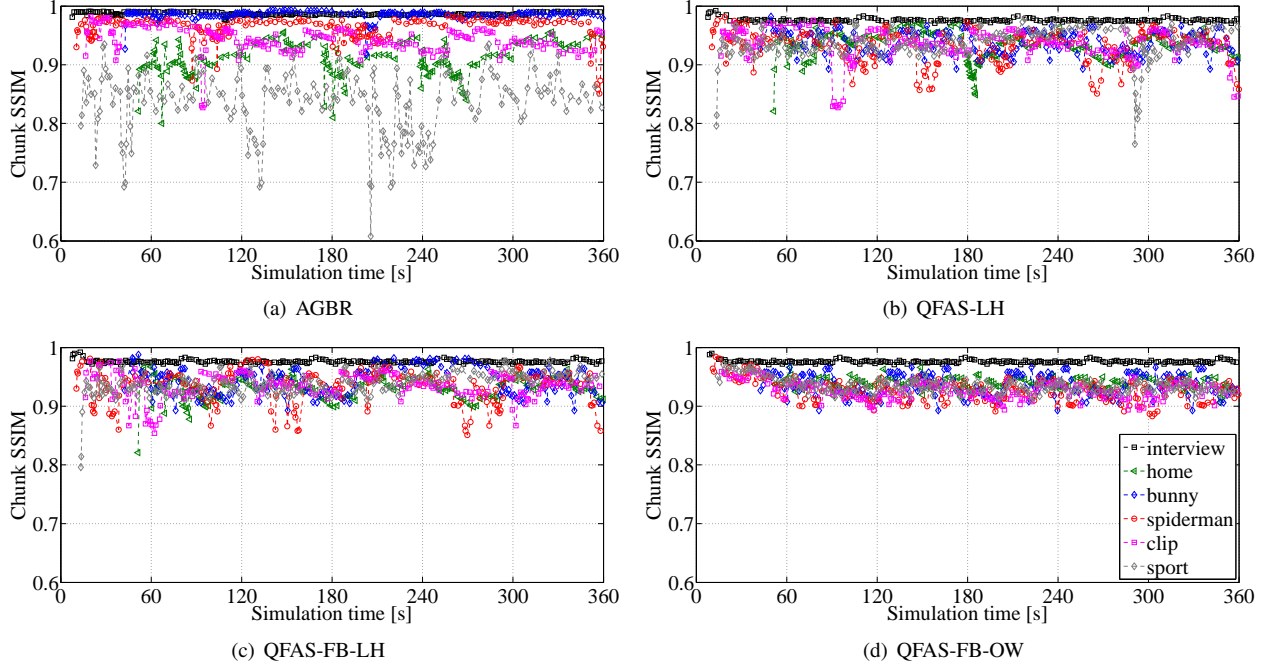
Fig. 6. An example (one drop of simulation) of the Chunk-by-chunk SSIM at the clients over time for the GBR-aware strategies.
