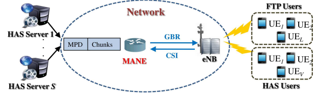
Fig. 1. System architecture.
