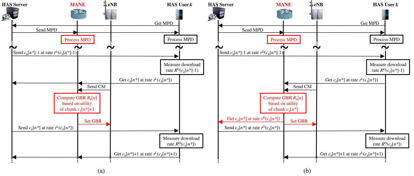
Fig. 2. Proposed approaches for a single HAS video delivery optimization: look-ahead strategy (a), and overwrite strategy (b). In the figure n^*T_s is the time instant at which chunk c_k is requested.
