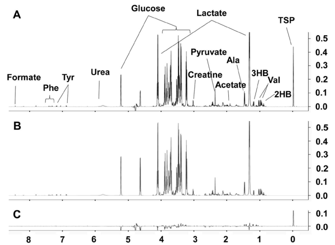
Figure 1 (A) ^1\text{H-NMR} serum spectrum with signal assignments. (B) ^1\text{H-NMR} spectrum of assigned metabolites. (C) difference spectrum (A, B). 2HB, 2-hydroxybutyrate; 3HB, 3-hydroxybutyrate; Ala, alanine; Gln, glutamine; Lys, lysine; Phe, phenylalanine; Tyr, tyrosine; Val, valine.
