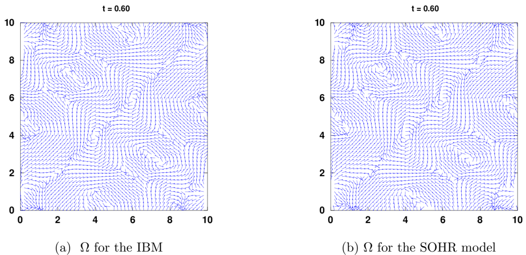
Figure 5: Mean direction \Omega for Taylor-Green vortex problem 4.12 at time t = 0.6s . Left: IBM. Right: SOHR model.
