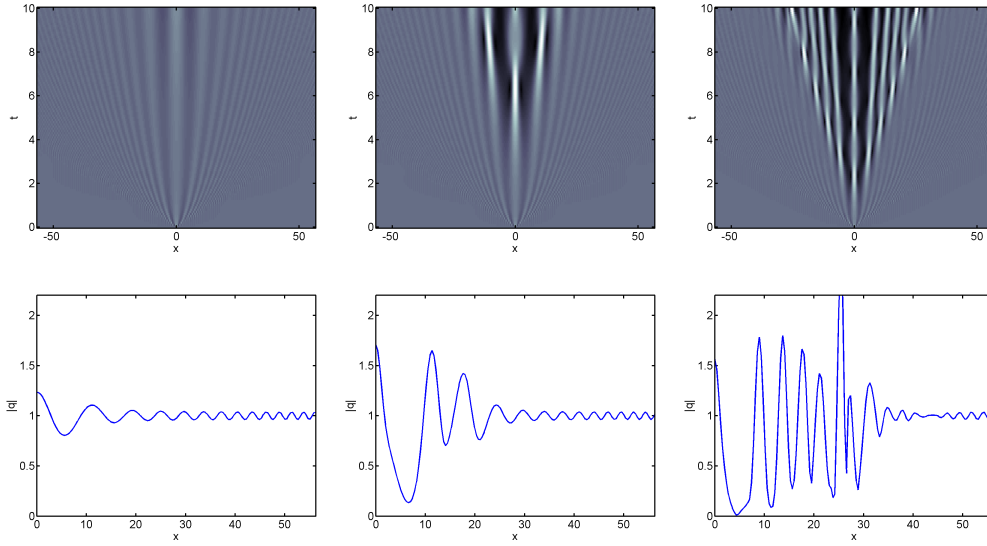
FIG. 9. Same as Fig. 7, but with s = 2 .
