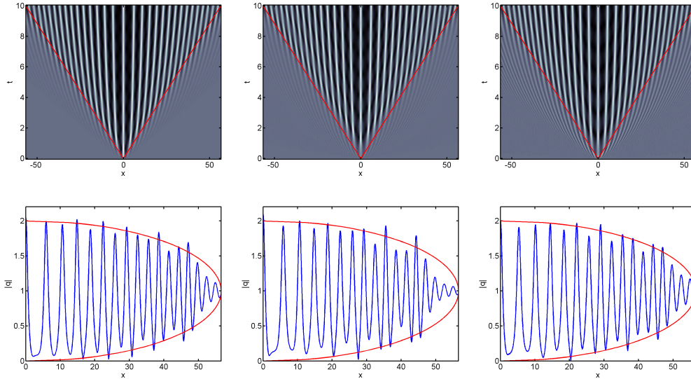
FIG. 1. Solutions of the focusing NLS equation starting from perturbations of a constant background. Top row: Density plot of |q(x,t)| , together with the predicted boundary (red lines) between the modulated oscillation region and the plane wave regions from [15, 16]. Bottom row: the solution |q(x,t)| at t = 10 (blue curve), together with the asymptotic envelope (red curve) from [15, 16]. Left column: Gaussian IC (8a); center column: sech-shaped IC (8b); right column: box-like IC (8c).
