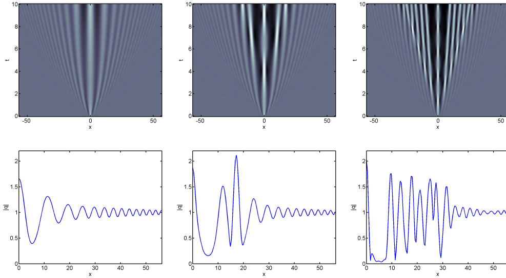
FIG. 10. Same as Fig. 8, but with s = 2 .
