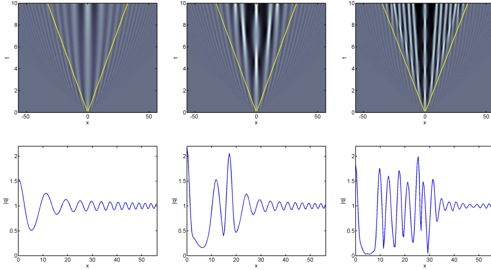
FIG. 5. Same as Fig. 3 but for s = 2 .
