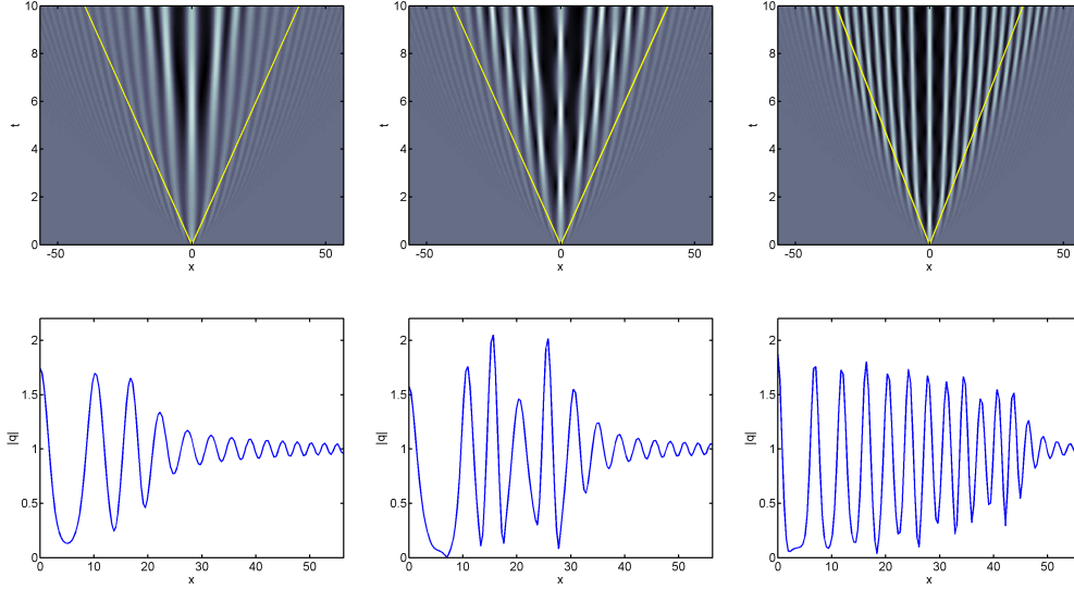
FIG. 3. Similarly to Fig. 1 with a Gaussian IC (8a) for the saturable nonlinearity model (left), the thermal media system (center) and the DMNLS equation (right), all with s = 1 .
