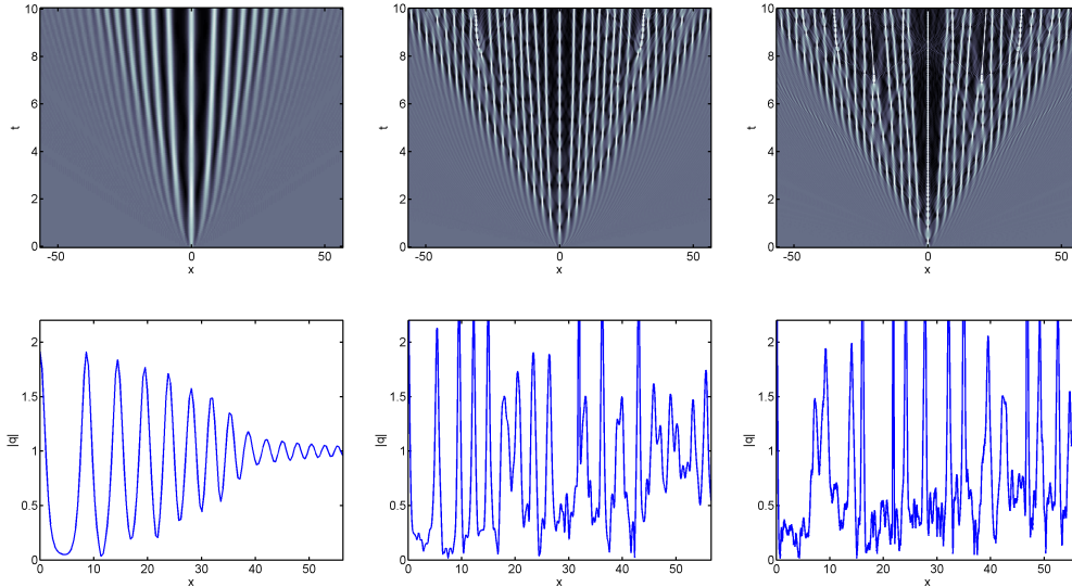
FIG. 6. Left column: evolution of a box-like initial perturbation (8c) of the constant background for the arbitrary power model (2), with \sigma = 1/2 . Center column and right column: evolution of a sech-shaped or box-like IC, respectively, for the same model with \sigma = 3/2 .
