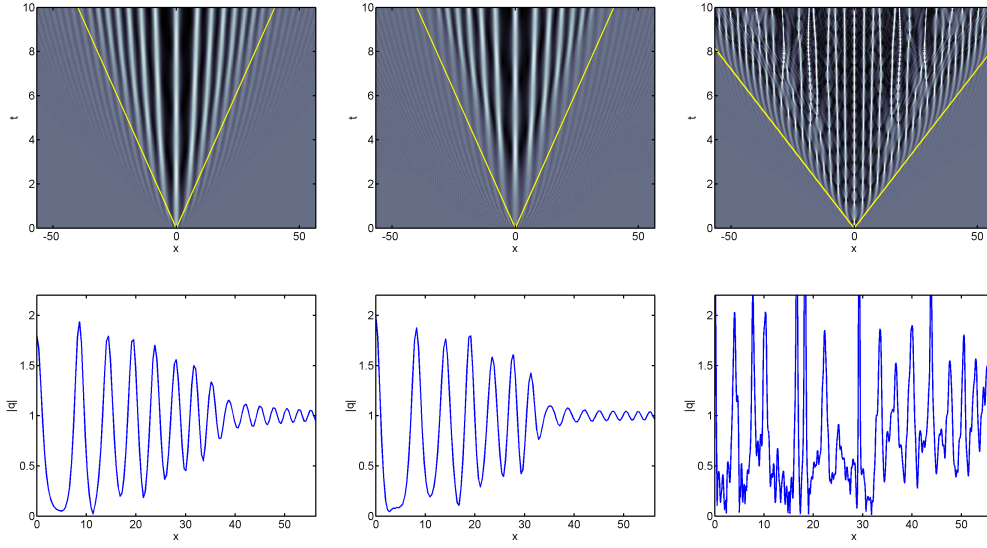
FIG. 2. Evolution of a Gaussian perturbation (8a) (left column) and a sech-shaped perturbation (8b) (center column) of the constant background, similarly to Fig. 1, but for the power-law model, (2), with \sigma = 1/2 , and a Gaussian IC (8a) with \sigma = 3/2 (right column). Yellow lines: the predicted boundary of the modulated oscillation region (see text for details).
