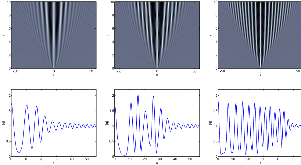
FIG. 8. Same as Fig. 7, but with a box-like IC (8c).
