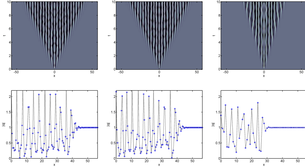
FIG. 12. Evolution of a Gaussian (left column) and a sech-shaped (center column) initial perturbation of the constant background for the DNLS equation with h = 1/2 . The right column shows the same Gaussian perturbation with h = 1 .
