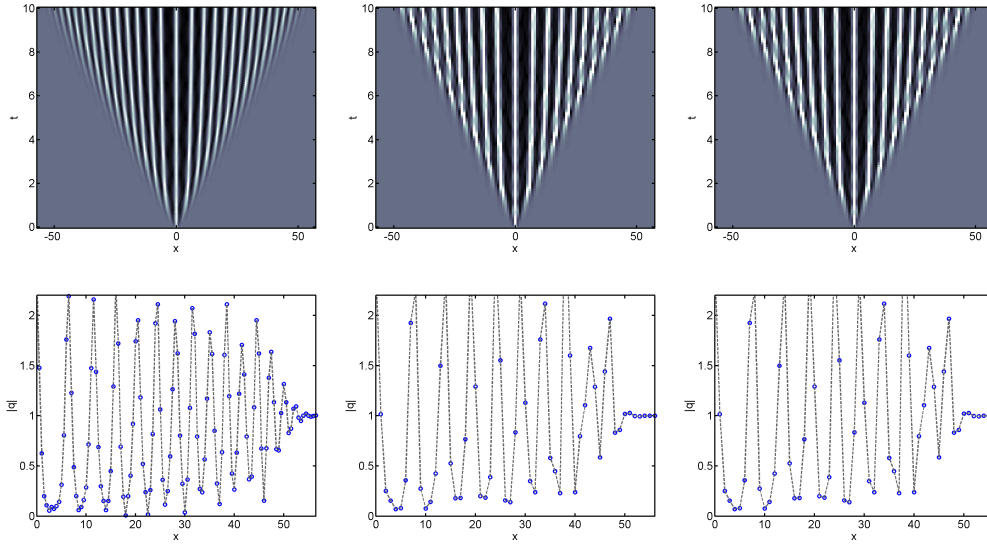
FIG. 11. Same as Fig. 6, but for the Ablowitz-Ladik equation, (7), with h = 1/2 (left column) or h = 1 (center and right columns).
