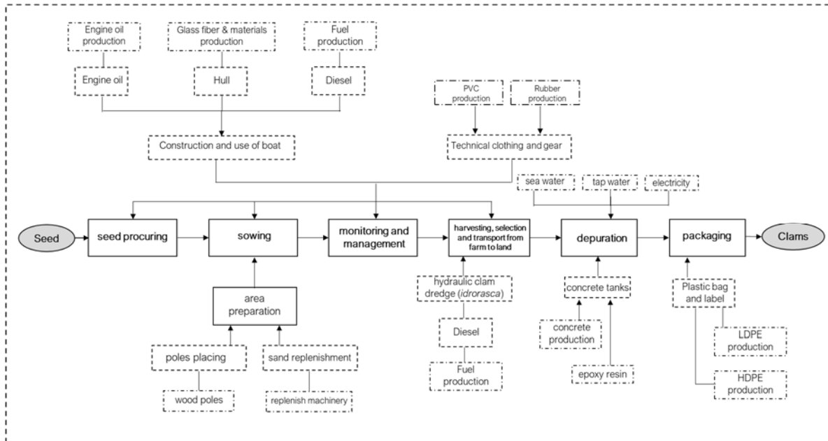
Figure 3. The system boundaries considered in this life cycle assessment (LCA) study. Foreground processes are depicted by solid boxes; background process by dashed boxes; raw materials, electricity, fuels and water production processes by dash-dotted boxes; mass flows by solid arrows; and products by grey circles. (PVC= polyvinylchloride; HDPE= high density polyethylene; LDPE= low density polyethylene).
