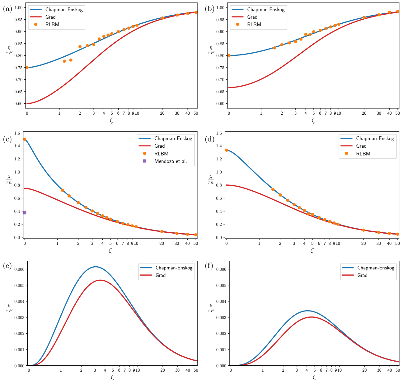
FIG. 1: Comparison of the non-dimensional transport coefficients for an ideal relativistic gas in (2+1) dimensions (left) and (3+1) dimensions (right, from [35]), obtained applying the Chapman-Enskog expansion and Grad’s method to the relativistic Boltzmann equation in the relaxation time approximation. For the thermal conductivity \lambda and the shear viscosity \eta we show the results of numerical measurements obtained using a lattice kinetic solver [8] which clearly rule in favor of the predictions of Chapman-Enskog. For the bulk viscosity \mu only the analytical results are available. We also show (panel (c)) the prediction for the ultra-relativistic thermal conductivity in (2+1) dimensions by Mendoza et al. in [60] obtained with Grad’s method, and differing by a factor two with respect to our calculations. Errors are of the order of 1% for all the numerical measurements (bars not shown).
