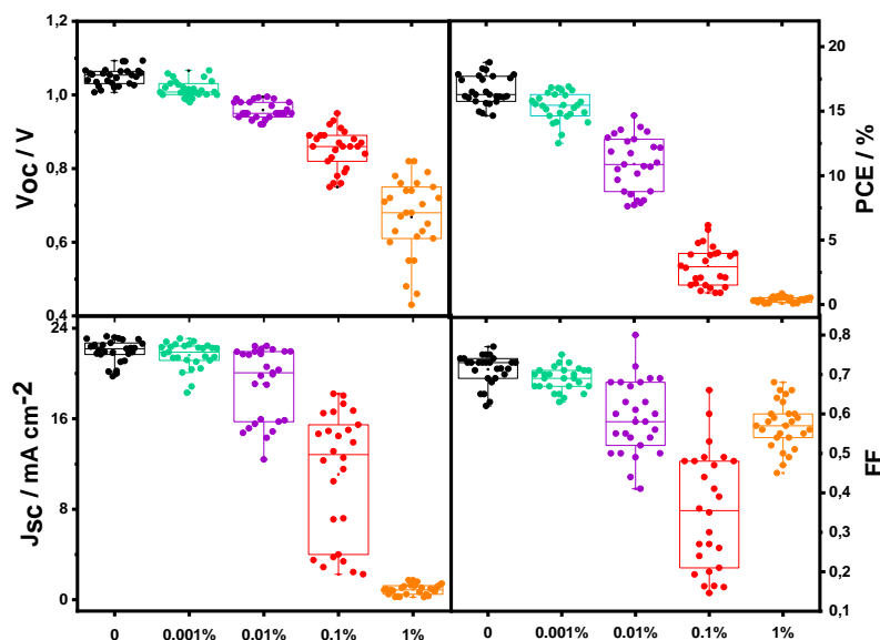
Figure 1. Characteristic parameters for solar cells containing different concentrations of intentionally added Bi denoted in at% referred to Pb. Even a concentration of 10 ppm results in a decrease of performance.
