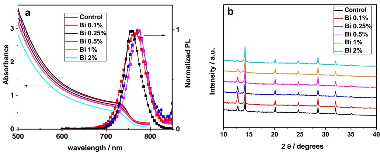
Figure 2. Characterization of thin films with different Bi content on glass (a) Absorption spectra, which are rather unaffected apart from a slight broadening of the onset. Normalized photoluminescence showing a slight red shift for higher Bi concentrations. (b) XRD data not showing any significant changes in the perovskite structure nor new phases.
