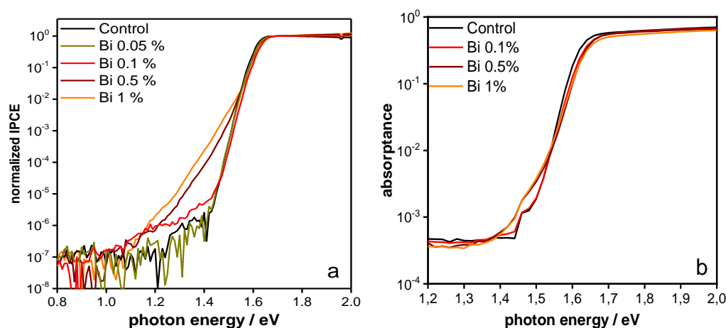
Figure 5. Sensitive optical measurements at the band edge (a) IPCE measured by FTPS and (b) PDS. Both measurements show that larger amounts of Bi introduce optically detectable tail states.
