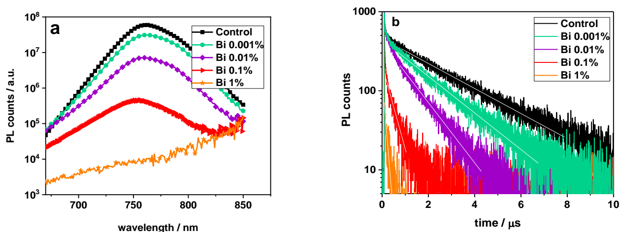
Figure 4. Photoluminescence of perovskite films (a) Absolute PL spectra showing that adding Bi reduces the PL yield so substantially that it is hardly detectable for [Bi] = 1%. (b) Transient PL with a reduced decay time for higher Bi concentrations. The white lines are mono-exponential fits and span the time range selected for the fits.
