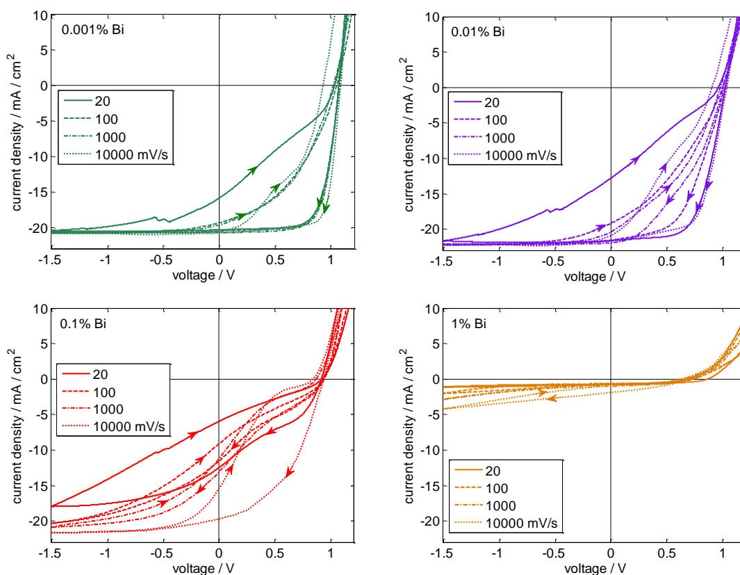
Figure 3. JV hysteresis loops starting from 1.2 V for various voltage sweep rates measured at solar cells with different Bi concentrations. Reduced J_{\text{SC}} and FF upon addition of Bi are mainly due to a strong dependence of charge extraction on the electric field. (The 0% Bi device behaves similarly as the 0.001%, see Fig. S2)
