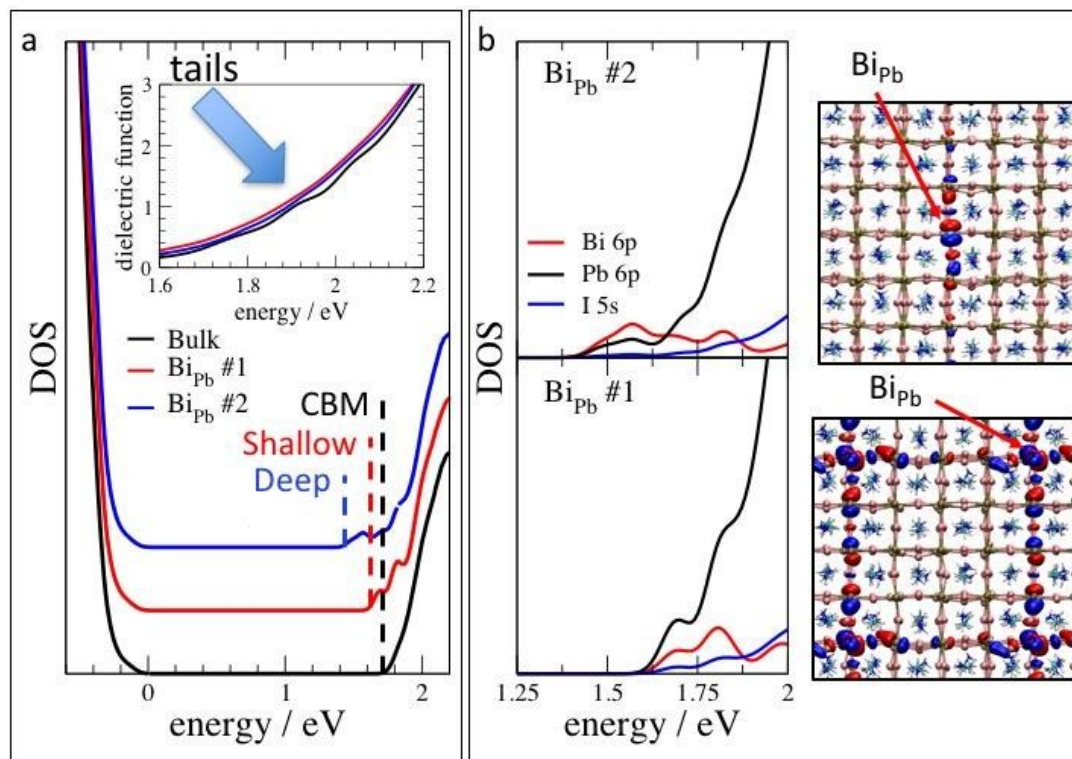
Figure 9. Results of theoretical calculations. (a) Density of state of the bulk (black) and two neutral Bi Pb defect configurations corresponding to shallow (red) and deep (blue) defect states. The zero of the energy axis is set to the valence band maximum (VBM). The lowest (half-filled) energy defect state of the first configuration overlaps with the bulk CBM. On the contrary, the corresponding state of the second configuration is well separated from the conduction band. In the inset it is reported the low energy part of the absorption spectrum, which shows the defect related low energy tails. (b) Contribution of Bi 6p, Pb 6p and I 5s atomic orbitals to the DOS in the energy range of defect states. On the right-hand side of the panel are reported the isosurface of the defect states of minimum energy. Isosurfaces are colored in blue and red according to the sign of the corresponding orbitals to put in evidence their antibonding character.
