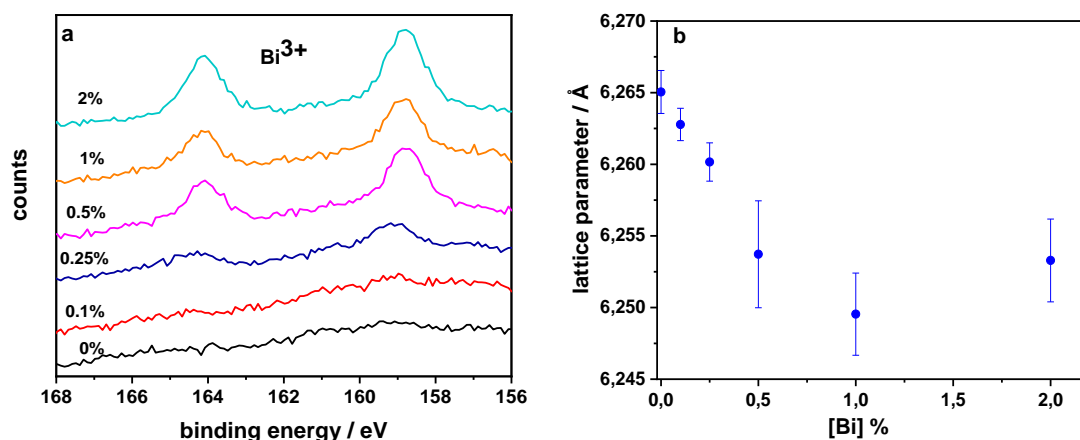
Figure 8. Structural characterization of perovskite films containing Bi (a) XPS spectra showing the characteristic signal for \text{Bi}^{3+} which increases for higher Bi content. (b) Lattice parameter deduced from fitting XRD spectra. Incorporation of Bi decreases the lattice parameter.
