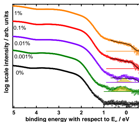
Figure 7. UPS measurements of \text{Cs}_{0.1}\text{FA}_{0.9}\text{Pb}(\text{Br}_{0.1}\text{I}_{0.9})_3 films with different Bi concentration (on ITO) showing the valence band region in a semi-logarithmic plot. For intermediate Bi concentration, a deep defect state (yellow) is observable which is superimposed by a broader density of states extending to the Fermi edge (black) for higher concentrations.
