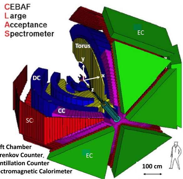
FIG. 3. A diagram of the CLAS detector, showing each of the six detectors.
