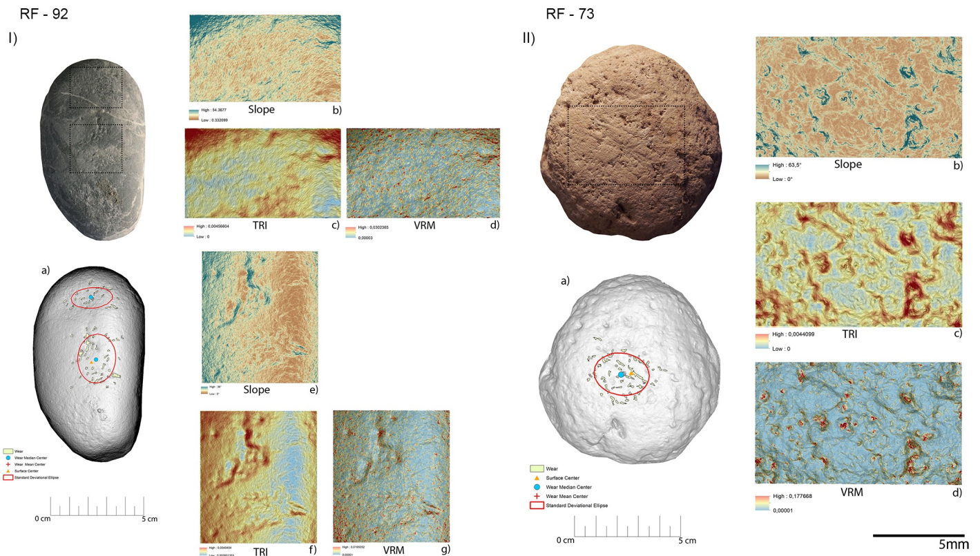
Fig 27. Archaeological items RF92 (I) and RF73 (II) utilized in retouch and percussion activities (RF92) and core ridge adjustment (RF73). (a) Spatial distribution of the identified wear; (b) slope; (c) terrain roughness index; (d) vector roughness measure.
