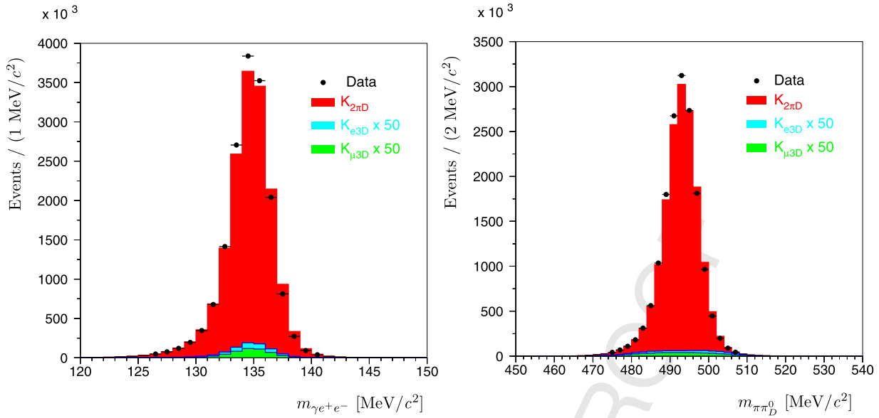
Fig. 1. Normalization candidates. Left: reconstructed \gamma e^+ e^- mass. Right: reconstructed \pi^\pm \pi^0 \pi^0 mass. Full dots correspond to data candidates; stacked histograms are, from bottom to top, the expected K_{\mu 3D} (green) and K_{e 3D} (blue) backgrounds multiplied by a factor of 50 to be visible. The normalization simulation (red) includes radiative effects in both kaon and \pi_D^0 decays that reproduce the asymmetric tails of both distributions.
