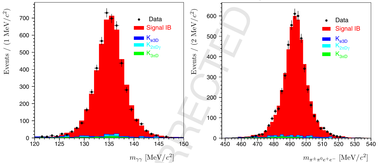
Fig. 2. Signal candidates. Left: reconstructed \gamma\gamma mass. Right: reconstructed \pi^\pm \pi^0 e^+ e^- mass. Full dots correspond to data candidates; stacked histograms are, from bottom to top, the expected K_{3\pi D} (green), K_{2\pi D\gamma} (light blue) and K_{e 3D} (dark blue) backgrounds and IB signal (red) estimated from simulation. All quoted errors are statistical.
