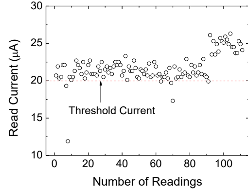
Fig. 7. Read variability of Forming current after the stop condition was reached.
