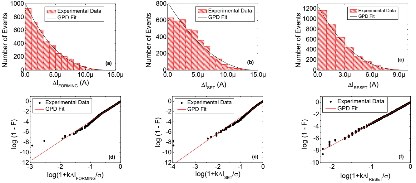
Fig 5. Histogram of the initial distribution of the Forming (a), Set (b), Reset (c) current shift and the corresponding cumulative distribution function (d,e,f). The observed linear behaviors of the cdf confirm that the three initial distributions follow a GPD.
