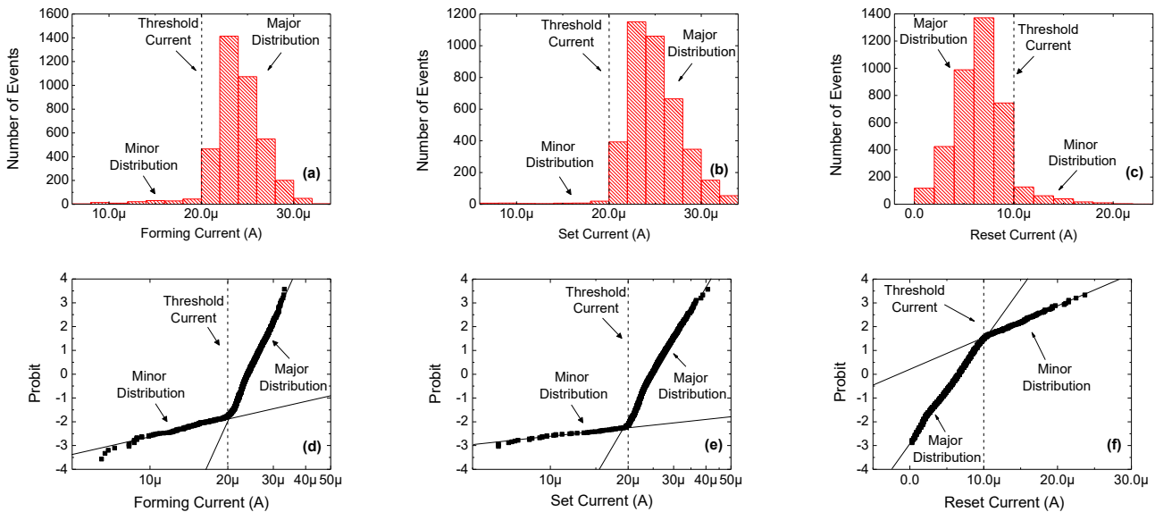
Fig 8. Histogram of the final distribution of the Forming (a), Set (b), Reset (c) current and the corresponding cumulative distribution function (d,e,f). A clear bimodal distribution is observed in all cases.
