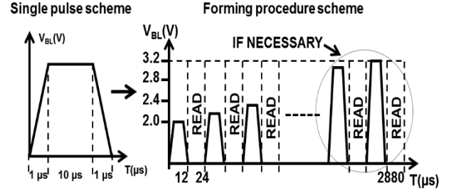
Fig. 3. IPV algorithm scheme.
