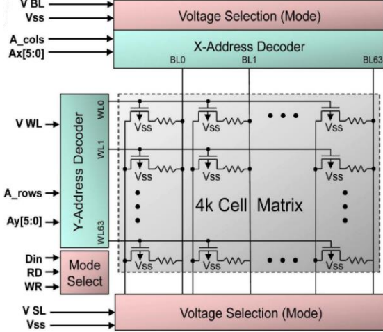
Fig. 1. Block diagram of the memory array.
