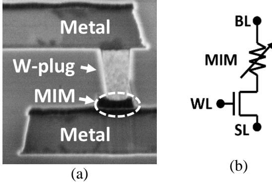
Fig. 2. Cross-sectional STEM image (a) and schematic (b) of the 1T-1R cell integrated in the arrays.
