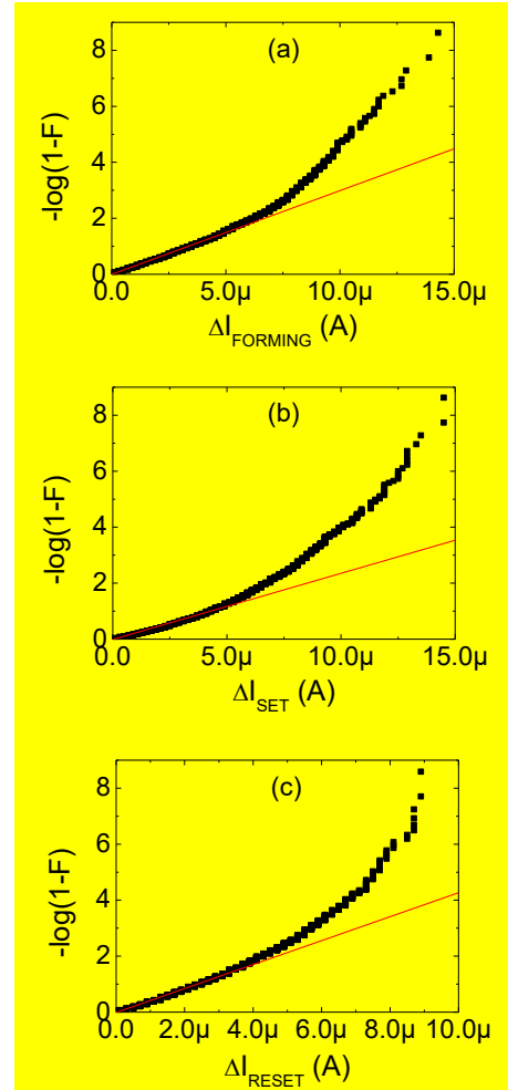
Fig. 6. The initial distribution of the Forming (a), Set (b), Reset (c) current shift do not follow an exponential distribution, as highlighted by the deviation of experimental data (symbols) by the linear behavior (red line).
