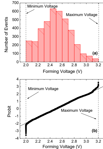
Fig. 4. Histogram of the forming voltage (a) and the corresponding cdf (b) in a normal probit scale. A normal distribution is observed in the explored voltage range.
