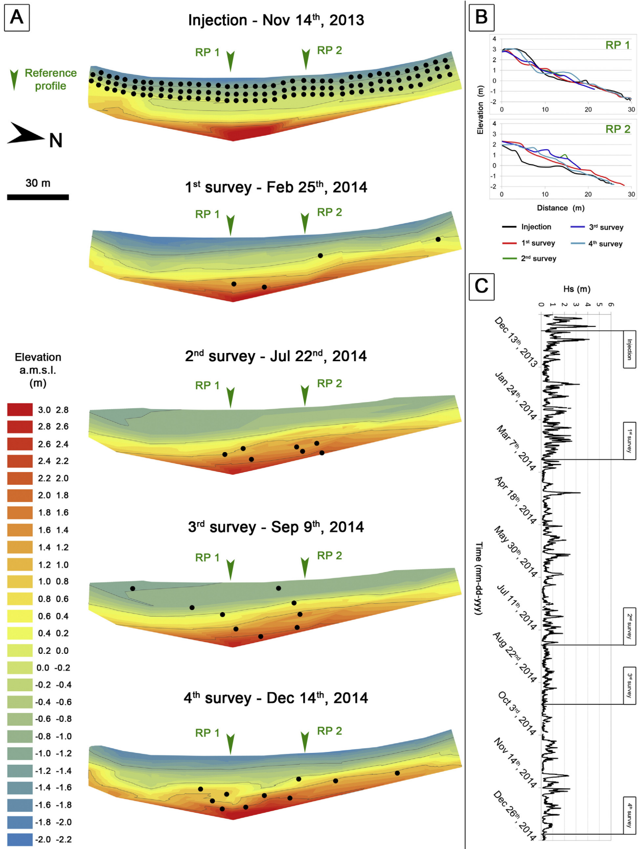
Fig. 3. The topographic maps show the geomorphologic evolution of the beach during the time frame of the experiment (a); the black dots represent the injection position and the recovery position of the tracers (the recovery position of the broken pebbles were not included in the maps). The evolution over time is also showed by overlapping the traces of two reference profiles, RP1 and RP2 (b). Plot showing wave height during the time frame of the experiment (c); wave data were provided by the Regional Hydrological Service.
