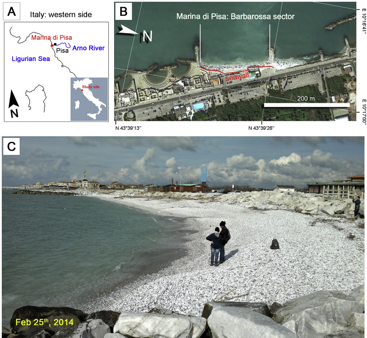
Fig. 1. The study site: a) geographic localization of Marina di Pisa (Tuscany, Italy); b) aerial view of the Barbarossa sector: the seawall at the back of the beach is evidenced with a red line (background image from Google Earth); c) southern view of Barbarossa beach (picture shot on 25th February 2014). (For interpretation of the references to color in this figure legend, the reader is referred to the web version of this article.)
