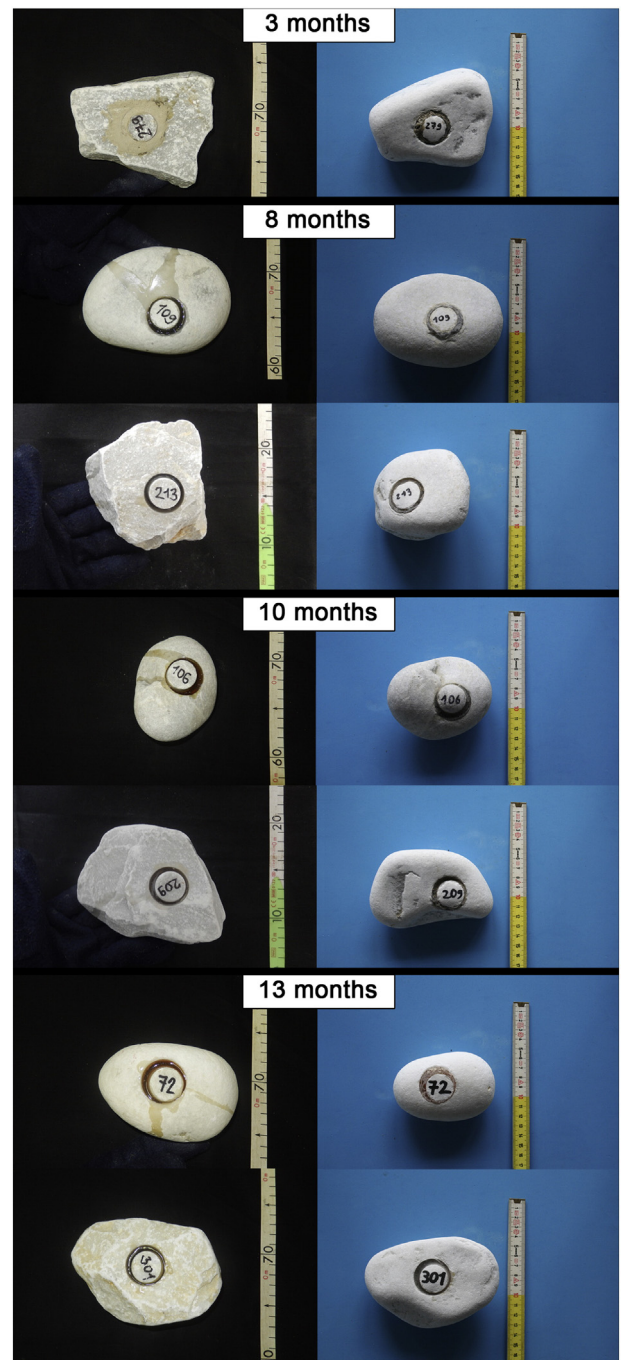
Fig. 2. Pairs of marked pebbles showing shape and roundness variations during each time interval (left column: initial configuration; right column: post-recovery configuration). Pairs of rounded and angular tracers are shown for each recovery campaign, except for the first campaign because the only rounded pebble that was recovered was discarded as it was clearly broken.
