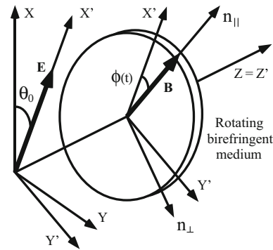
Fig. 3 Reference frame for the calculations. XY : laboratory coordinates; X' : direction of the electric field as defined by the polariser; n || : direction of the magnetic field, rotating around the beam path Z at a frequency \nu_B
