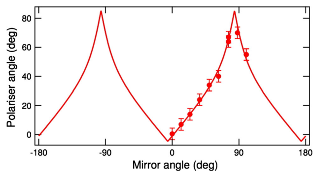
Fig. 9 Polariser angle as a function of the azimuthal angle of the mirror in a Cotton–Mouton measurement of 230 \mu\text{bar} of Ar. Data are fitted with \phi_{\text{EQ}} as given by Eq. (25)
