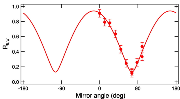
Fig. 8 Rotation-to-ellipticity signals ratio plotted as a function of the azimuthal angle of the input mirror in a Cotton–Mouton measurement of 230 \mu\text{bar} of Ar gas. The fit line is the (N/2) -amplified phase difference \alpha_{\text{EQ}} of the equivalent wave-plate of the mirrors given by Eq. (24)
