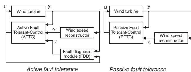
Figure 11. Structures of the active and passive fault-tolerant control systems.
