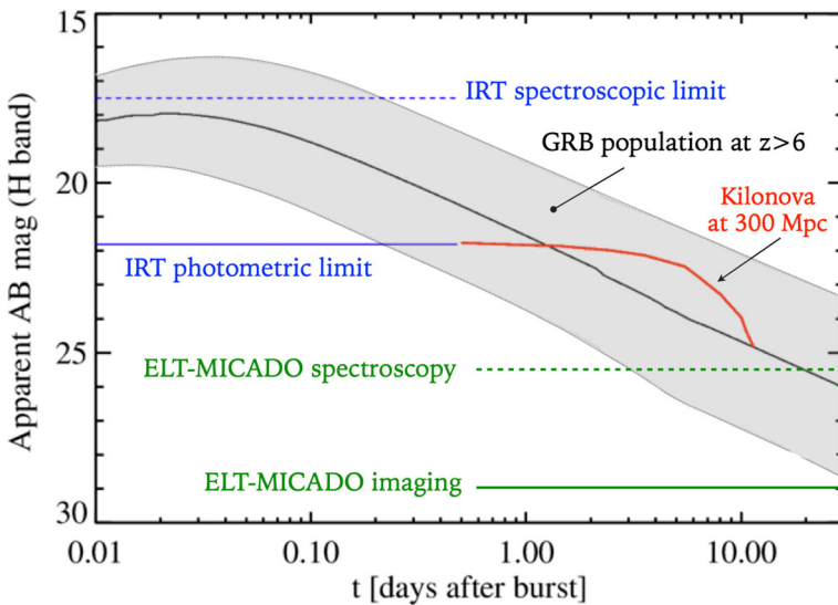
Fig. 3 Expected H-band light curves of the afterglow of high redshift GRBs and a kilonova from NS-NS merger at 300 Mpc. The shaded area indicates the median (black line) and 1\text{-}\sigma scatter of 100 simulated light curves drawn from GRB population models at z > 6 following [11]. The red curve represents the kilonova associated to GW170817, projected to a distance of 300 Mpc, using H-band photometry from [12]. Horizontal lines indicate the limiting magnitude of THESEUS IRT (600s and 1800s exposure for photometric and spectroscopic limit, with SNR= 5 and 3, respectively,) and ESO ELT-MICADO (1 h exposure with SNR = 5) in imaging and spectroscopic mode respectively (re-adapted from [13])
