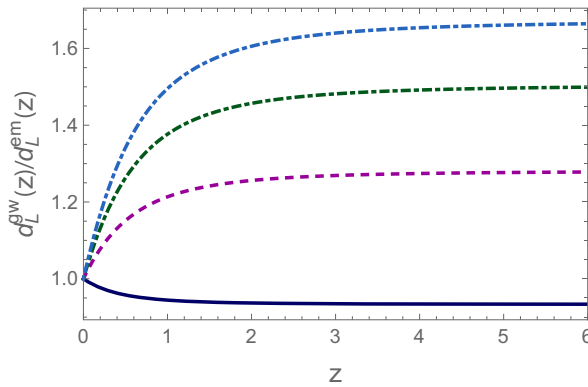
Fig. 8 Example of the ratio of the gravitational to electromagnetic luminosity distance in a modified gravity model, for different values of a parameter related to the energy scale of inflation. In the upper curve, the deviations of d_L^{gw}(z) from d_L^{em}(z) reaches 60% at large redshift (from [69])
