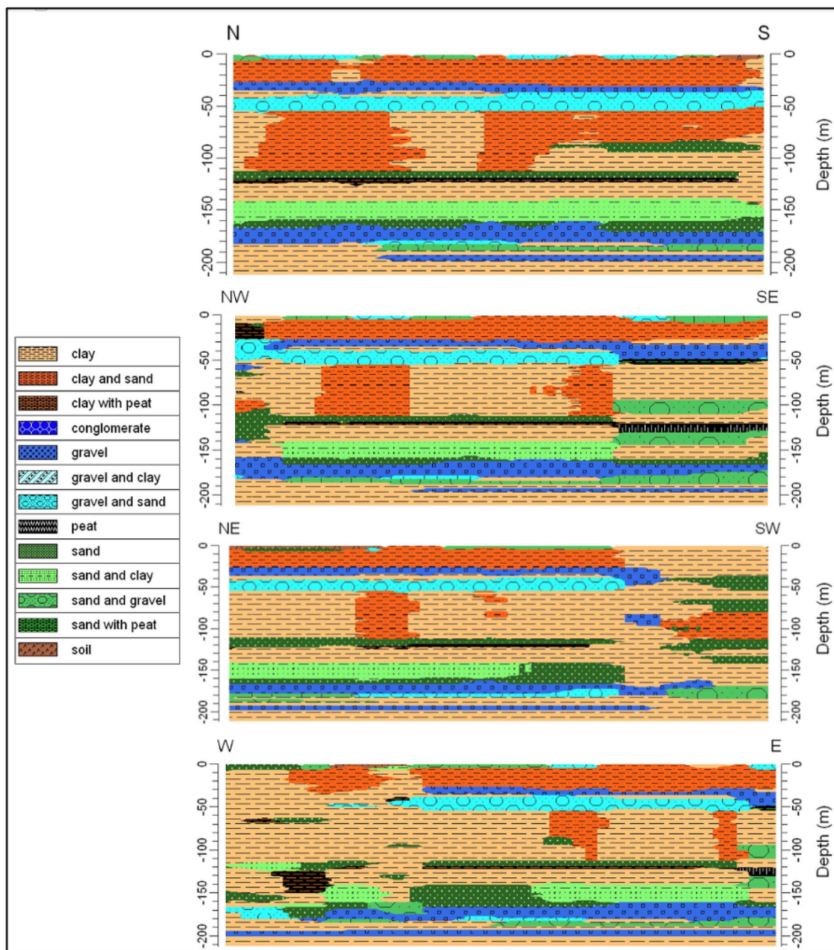
Fig. 3 2D lithostratigraphic sections extrapolated from the lithological model
