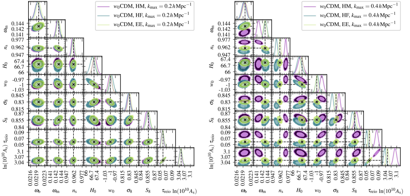
Figure 7. w_0 CDM cross comparison of HMCode and HALOFIT vs EuclidEmulator1 considering k \leq 0.2 h \text{Mpc}^{-1} (left triangle plot) and k \leq 0.4 h \text{Mpc}^{-1} (right triangle plot), respectively. Just as in Fig. 6 we see good agreement between the posteriors in the case with the lower cut-off scale while increasing that scale leads to emergent differences.
