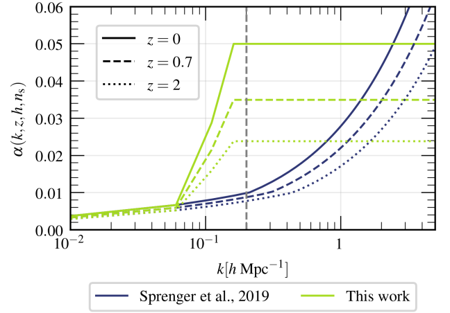
Figure 3. The two different envelope functions \alpha for theoretical uncertainty as defined in Eq. 3. The solid, dashed and dotted lines indicate the uncertainty envelope at redshifts z = 0 , z = 0.7 and z = 2 , respectively, where [0.7, 2] is the redshift range of the Euclid likelihood. Blue lines indicate the original theoretical uncertainty \sigma_{\text{th,S}} from Sprenger et al. (2019) and green lines correspond to \sigma_{\text{th,KB}} , a rough estimate of the agreement between EuclidEmulator1 and HMCode, as described in the text in section 2.4. The vertical dashed grey line indicates k = 0.2 h \text{ Mpc}^{-1} which is a popular choice for the upper k cut-off value. In most cases, we use the theoretical uncertainty \sigma_{\text{th,S}} , but at the end we compare to the other uncertainty for a cross-comparison case.
