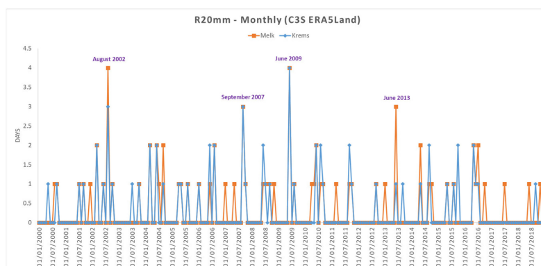
Figure 7. Time series (2000–2018) relating to R20mm (number of days in a month with precipitation greater than or equal to 20 mm/day) values extracted from C3S ERA5 Land monthly scale for Krems and Melk.
