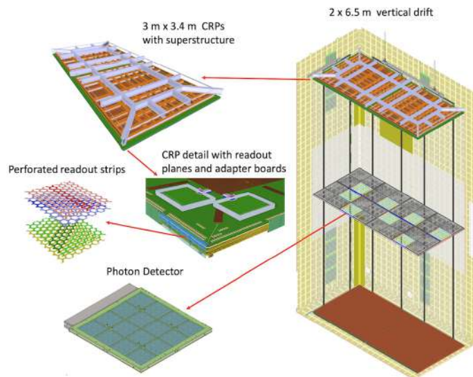
Figure 8. Schematic of the vertical drift FD2 concept with PCB-based charge readout. Corrugations on cryostat wall shown in yellow; PCB-based CRPs (brown, at top and bottom with superstructure in gray for top CRPs); cathode (violet, at mid-height with openings for photon detectors); field cage modules (white) hung vertically around the perimeter (the portions near the anode planes are 70% optically transparent); photon detectors (light green at right), placed in the openings on the cathode and on the cryostat walls, around the perimeter in the vertical regions near the anode planes. Reproduced from [60]. The Author(s). CC BY 4.0.
