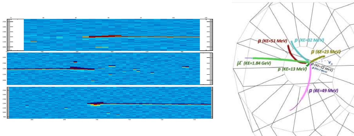
Figure 26. The same \text{CC } \nu_\mu event with seven low energy protons (kinetic energies ranging from 7 to 51 MeV) simulated in a \text{LArTPC} (left) and a \text{GARrTPC} (right). The \text{LArTPC} event display shows time ticks versus channel number for the three projective views of the event. The \text{GARrTPC} reconstruction algorithm finds all eight tracks in the event (seven proton tracks and one muon track), although only six are visible by eye in this view. All proton tracks travel 2.4 cm or less in \text{LArTPC} . Reproduced with permission from [109].
