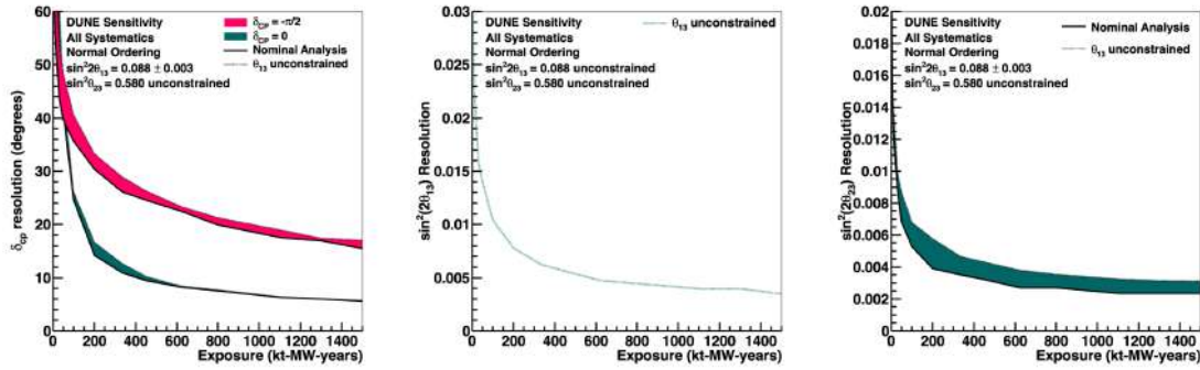
Figure 3. The resolutions to \delta_{CP} (left), \sin^2 2\theta_{13} (center), and \sin^2 \theta_{23} (right), shown as a function of exposure in kt-MW-yrs, assuming the full constraint from the ND, including MCND. The ultimate precision of DUNE requires an exposure greater than 600 kt-MW-yrs, which requires FD3 and FD4 to be built in a reasonable timescale. Reproduced from [8]. CC BY 4.0.
