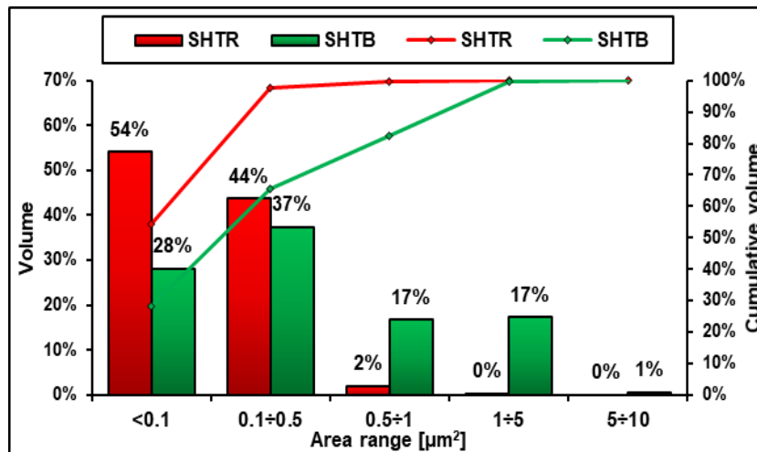
Fig. 10. Area distribution of Si particles for SHTR ( T_{\text{SHT}}=510 \text{ °C} and t_{\text{SHT}}=10 \text{ min} ) and SHTB ( T_{\text{SHT}}=540 \text{ °C} and t_{\text{SHT}}=1 \text{ h} ) conditions.
