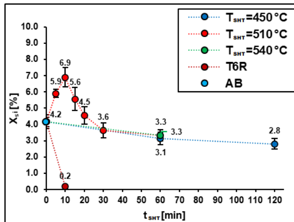
Fig. 5. Amount of Si dissolved in FCC Al ( X_{Si} ) estimated by Vegard's law for SHTed samples with different T_{SHT} and t_{SHT} and for a T6R heat-treated sample.
