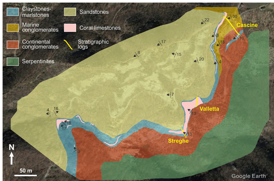
Fig. 2. Detailed geological map of the study area with indication of the three measured stratigraphic sections.
