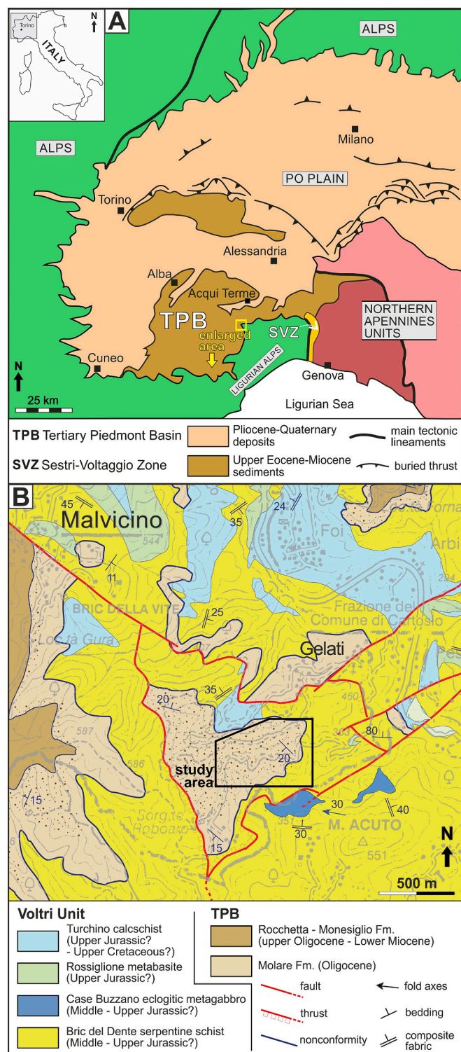
Fig. 1. A. Simplified structural map of north-west Italy (modified from Dela Pierre et al., 2010). B. Geological map of the Gelati surroundings and location of the study area (modified from Federico et al., 2022).
