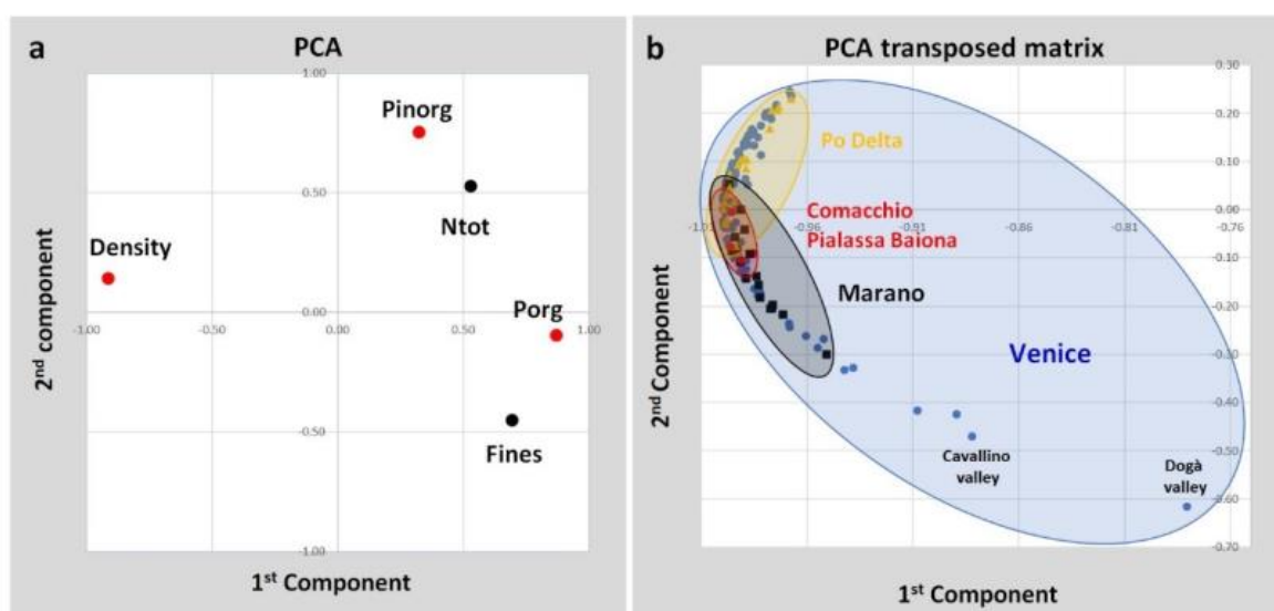
Figure 5. (a) PCA among nutrient species, sediment density and grain size (fines). Red circles represent values of loading > 0.7. (b) PCA of the transposed matrix to highlight the station and lagoon associations. The different colors show different TWSs. Blue circles: Venice lagoon; black squares: Marano-Grado lagoon; other triangles: Po Delta lagoons and ponds; in red: Comacchio valleys and Pialassa della Baiona.
