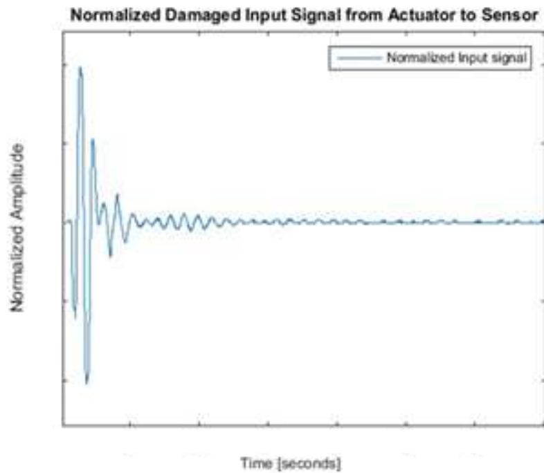
Figure 54. Excitation signal
