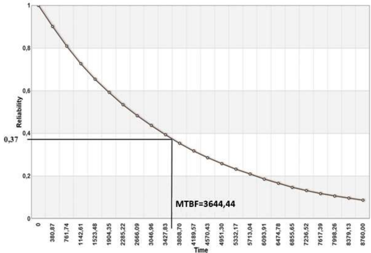
Figure 25. Reliability through time in a year operation
