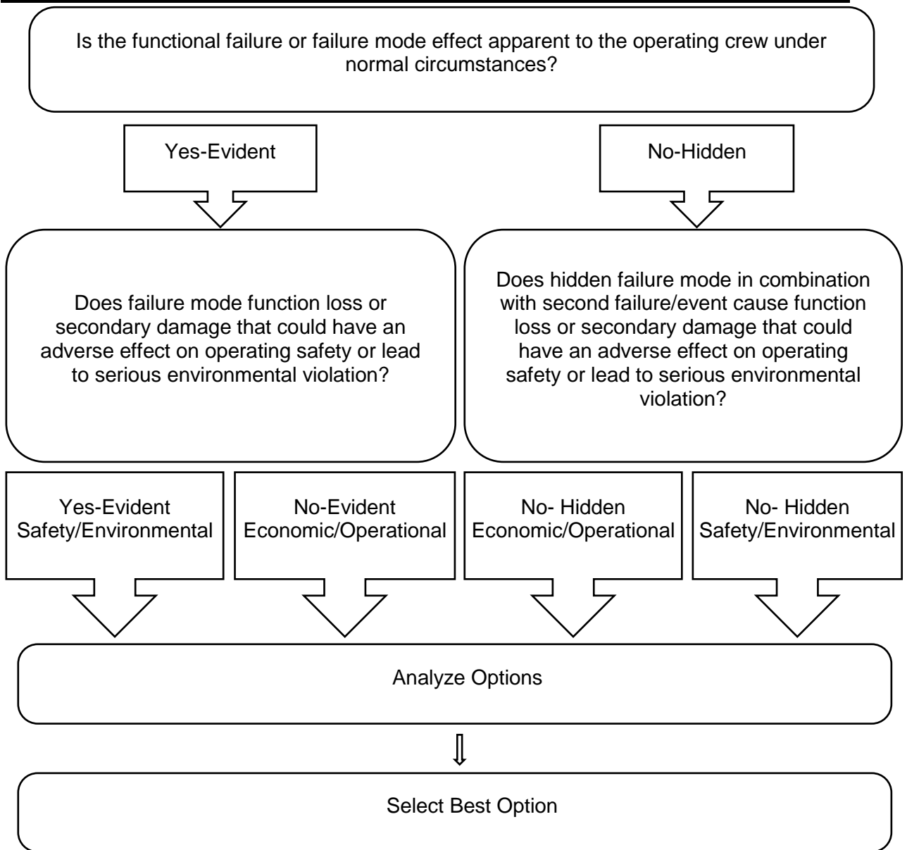
Figure 42. Decision Logic
