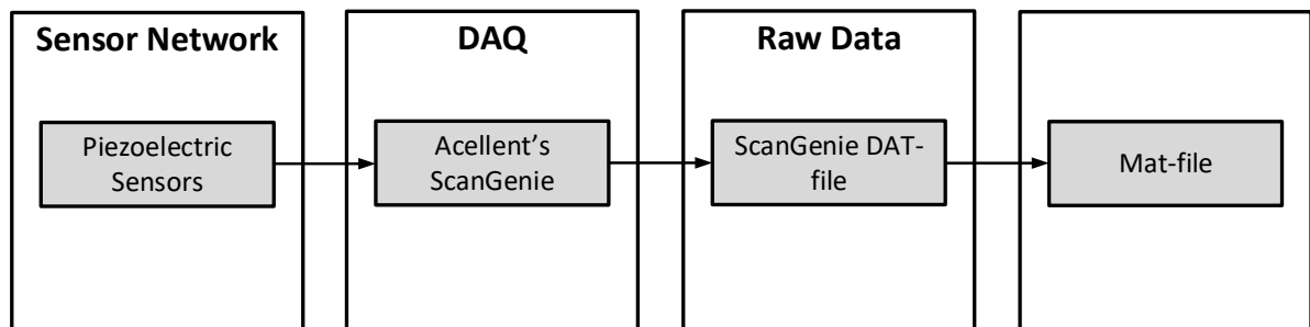
Figure 52. Flowchart data acquisition system
