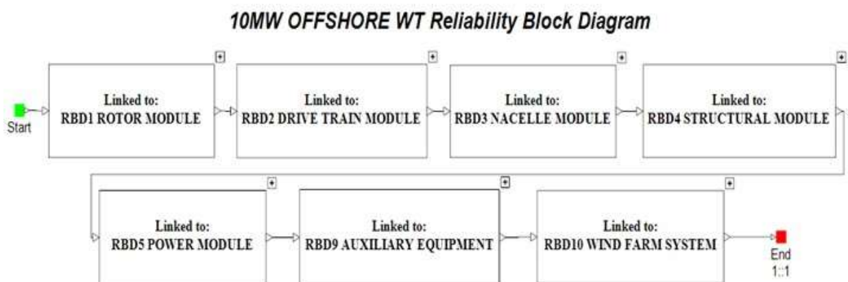
Figure 20. Main RBD of the Offshore Wind Turbine
