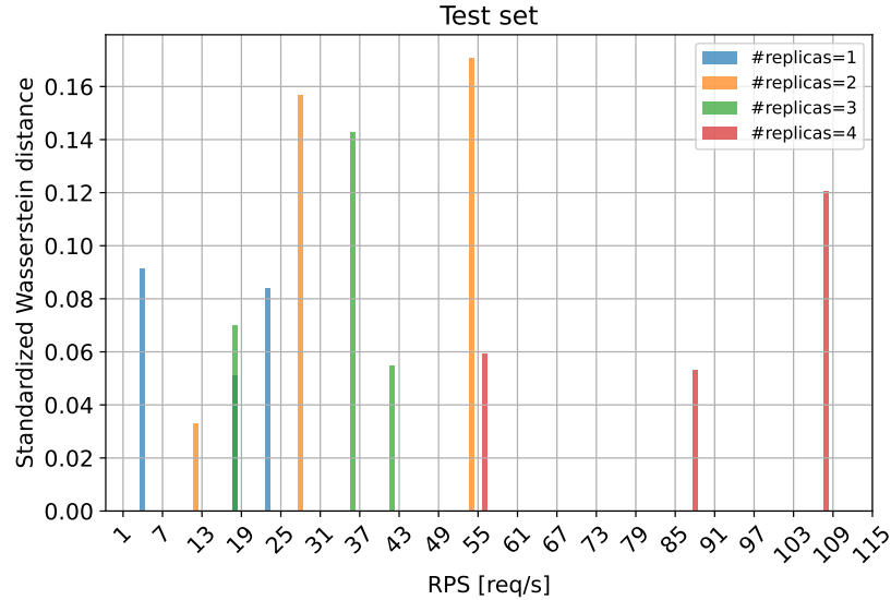
Figure 6.19: Performance evaluation of MDN model for MS1 in terms of Standardized Wasserstein metric on the test set.
