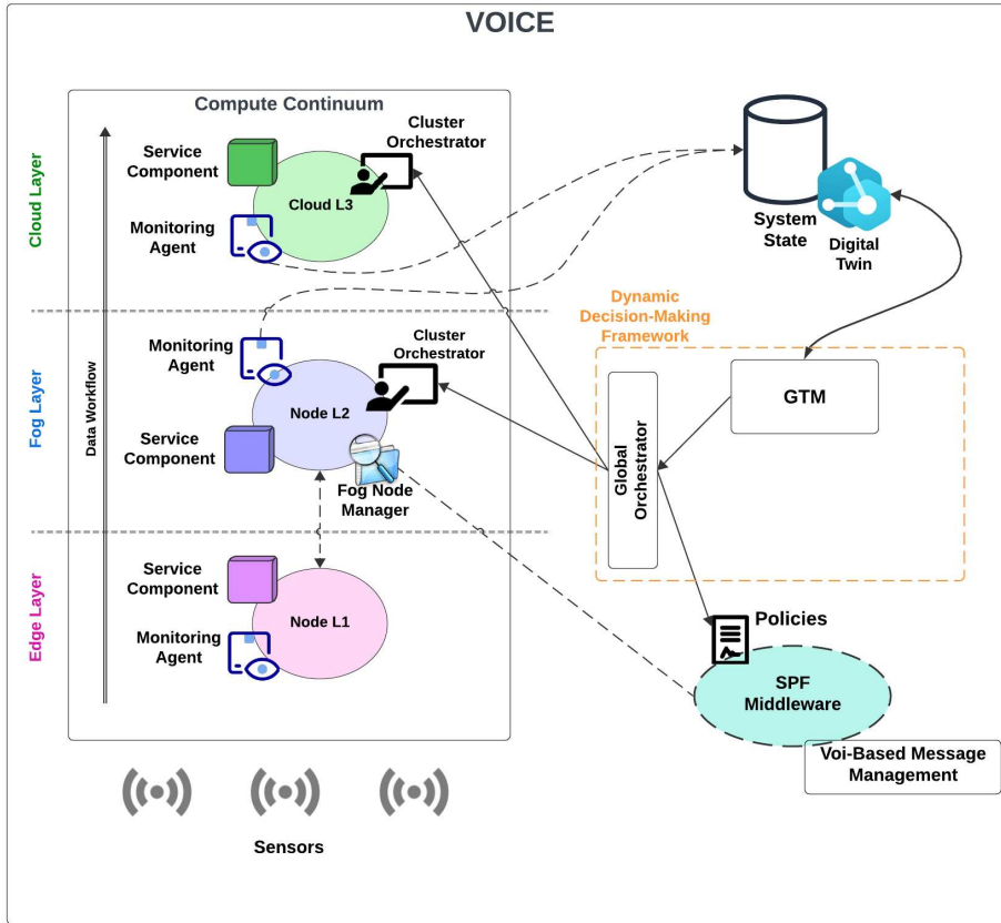
Figure 4.3: Global picture of the VOICE architecture
