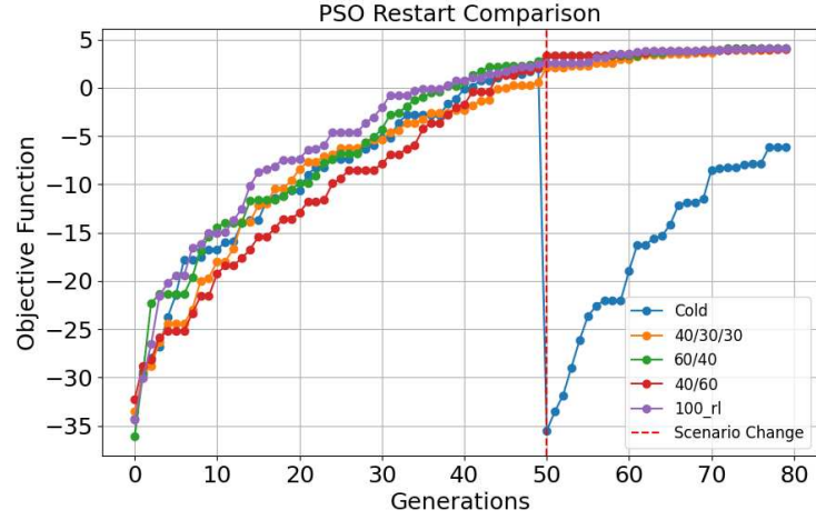
Figure 4.9: Exploitation of cold and hot restart approaches for PSO algorithm.
