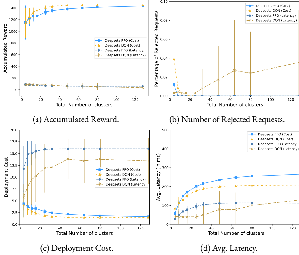
Figure 5.6: The results for the trained DS agents for both reward functions while varying the number of available clusters.
