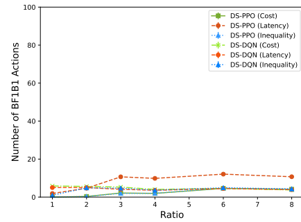
(h) Best Fit (BF1B1) Actions.
