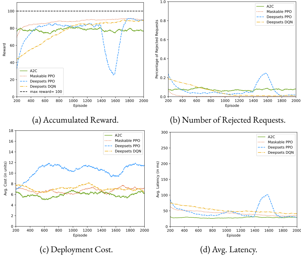
Figure 5.5: The training results for the several evaluated agents for the latency reward function.
