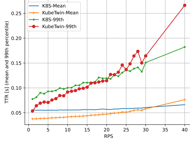
Figure 6.8: The distribution of the mean TTR value for 5000 requests under different RPS values using a 3 replicas deployment and the RPS 20 model.
