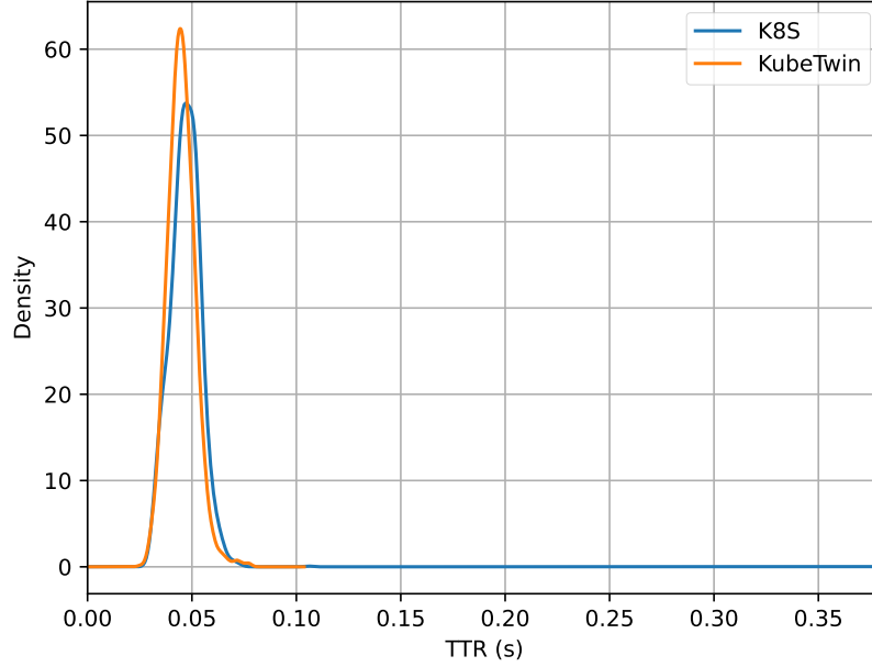
Figure 6.4: The results of the simulation-based inference process.
