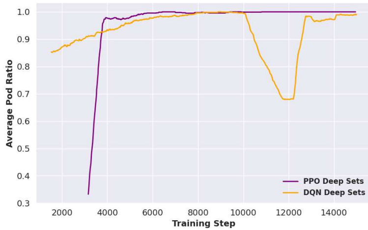
Figure 7.6: Average pod ratio during training.
