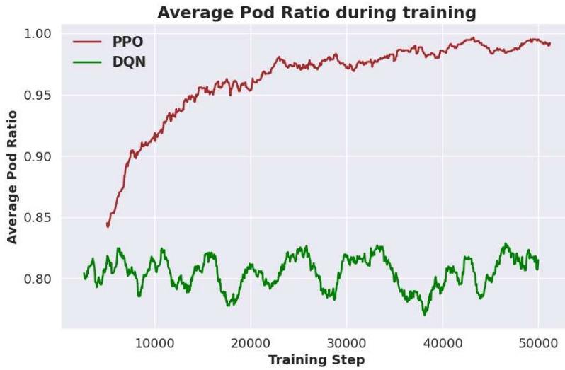
Figure 7.4: Average DQN and PPO Pod Ratio in 50000 steps of training.
