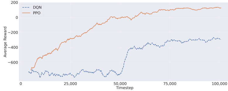
Figure 4.1: The DQN and PPO mean reward during the training process.
