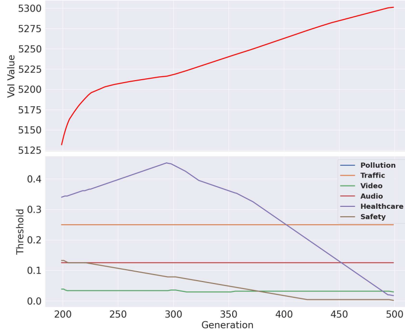
Figure 4.6: Total VoI evolution in relation to the service thresholds manipulation by QPSO.
