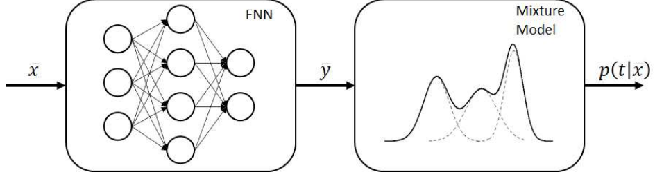
Figure 6.9: Structure of a MDN.
