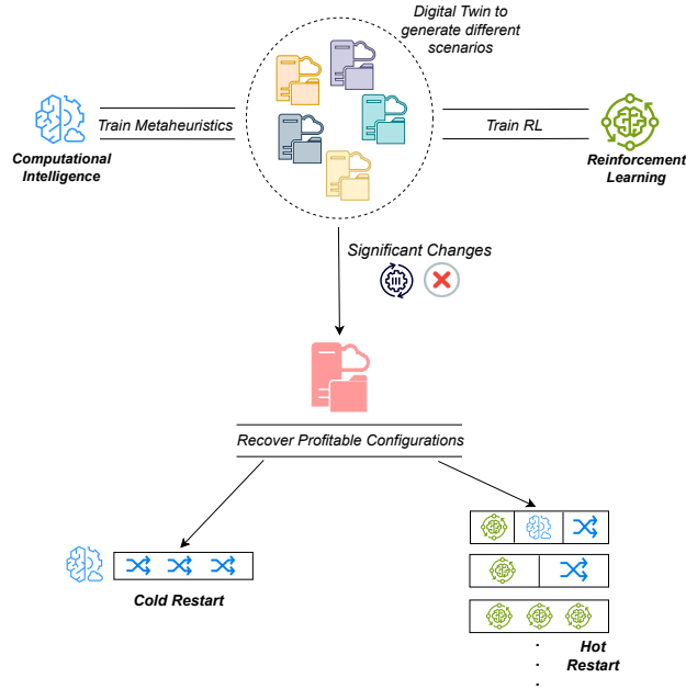
Figure 4.7: Exploitation of cold and hot restart approaches.
