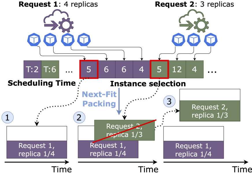
Figure 5.15: Scheduling and Resource Allocation decisions taken with MOEA. The encoding vector is divided into two parts: the first decides the scheduling for each request, and the second assigns each replica to a proper instance type (DC, type, size), encoded as an integer. Then, instances are created according to a next-fit algorithm: replicas are packed sequentially, and new instances are opened as soon as the capacity is exceeded.
