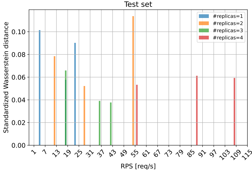
Figure 6.20: Performance evaluation of MDN model for MS2 in terms of Standardized Wasserstein metric on the test set.
