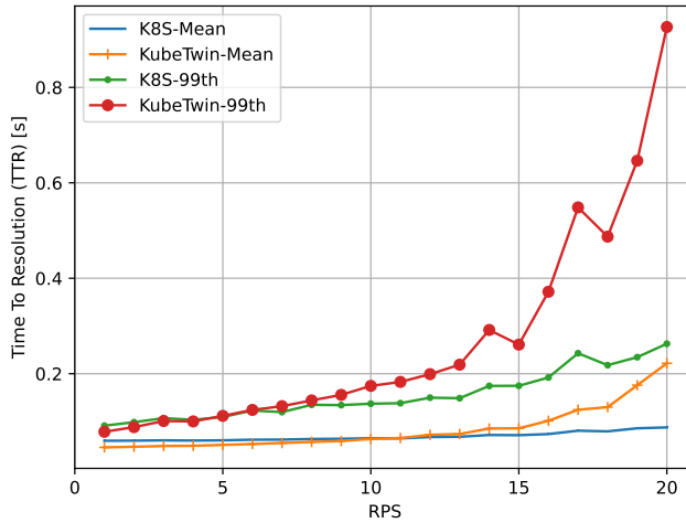
Figure 6.5: The average and the 99th percentile TTR values collected for 5000 requests with KubeTwin and the K8S under different workload RPS.
