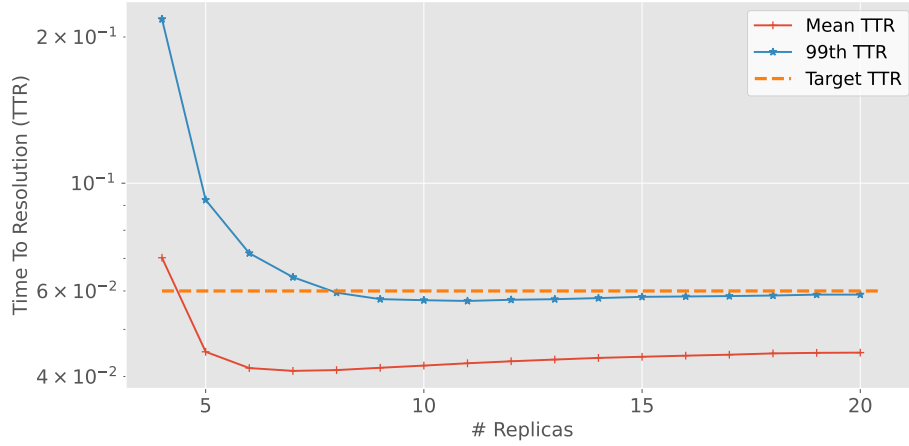
Figure 6.24: Mean and 99th percentile TTR at different numbers of replicas
