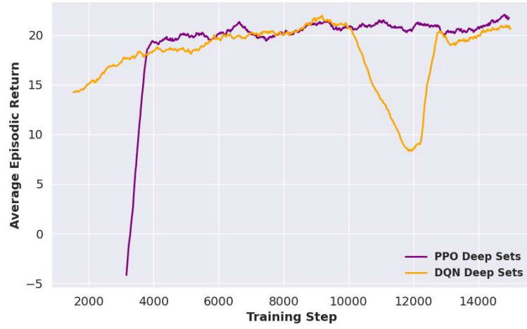
Figure 7.5: Average episodic return during training.
