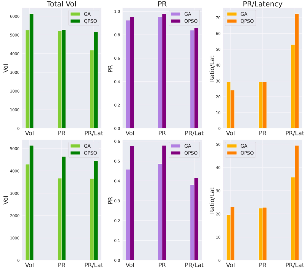
Figure 4.4: Results of the three different optimization methodologies using GA and QPSO as optimization algorithms.
