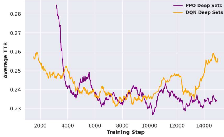
Figure 7.7: Average TTR during training.
