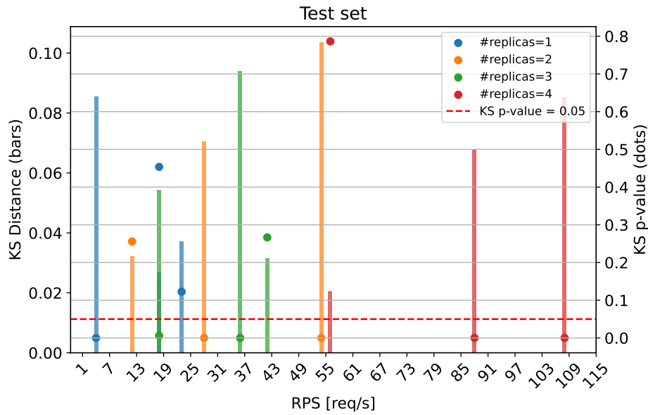
Figure 6.17: Performance evaluation of MDN model for MS 1 in terms of Kolmogorov-Smirnov on the test set.
