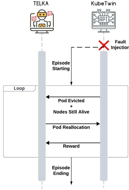
Figure 7.1: The workflow between TELKA and KT. TELKA tries to reallocate evicted pods due to injected faults.
