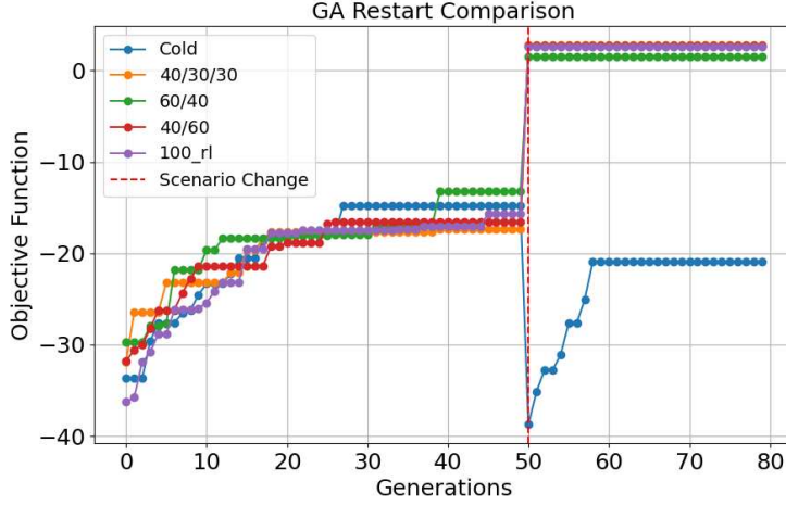
Figure 4.8: Exploitation of cold and hot restart approaches for GA algorithm.
