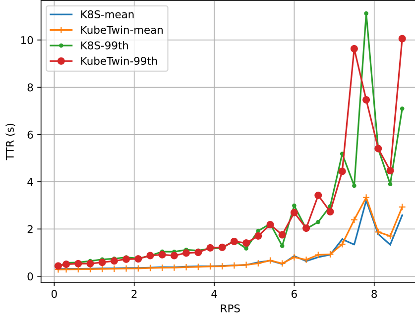
Figure 6.22: Comparison between the mean and 99th percentile response time of the real application and KT, with sd = 10 and 3 replicas for each microservice.
