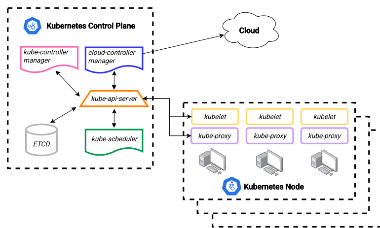
Figure 5.1: High-level figure of the Kubernetes infrastructure.
