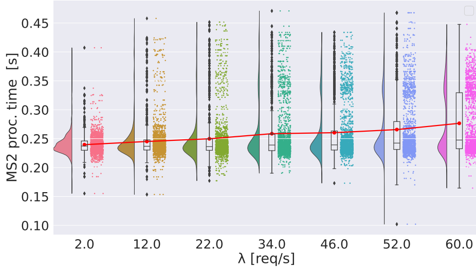
Figure 6.16: Raincloud plot of MS2 proc. time, conditioned to RPS, for sd = 10x and two replicas (non threaded).
