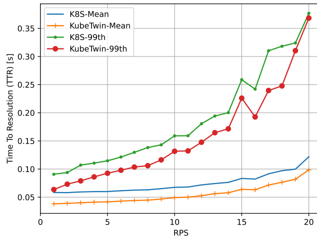
Figure 6.7: The average and the 99th percentile TTR values collected for 5000 requests using the model Fitted at RPS 20.
