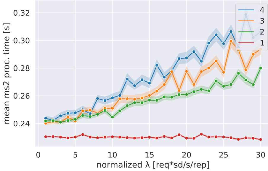
Figure 6.15: Comparison of MS2 mean proc. time (95% confidence interval) for sd = 10x . The processing time is plotted for different combinations of RPS values and numbers of replicas. The RPS ( \lambda ) is equally balanced among replicas.
