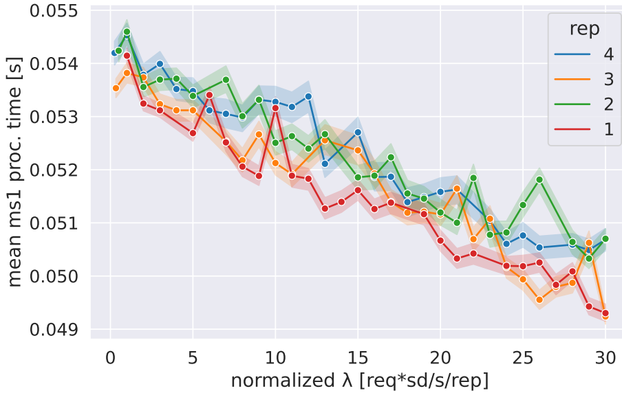
Figure 6.13: Comparison of MS1 mean proc. time (95% confidence interval) for sd = 10x . The processing time is plotted for different combinations of RPS values and numbers of replicas. The RPS ( \lambda ) is equally balanced among replicas.
