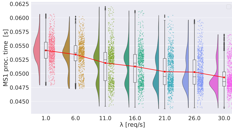
Figure 6.12: Raincloud plot [250] of MS1 proc. time, conditioned to RPS, for sd = 10 and one replica (non threaded).
