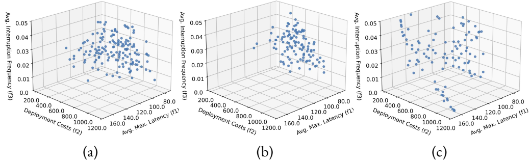
Figure 5.17: PFs found by NSGA-II, NSGA-III, and MPSO, considering total deployment costs, avg. request maximum latency and avg. interruption frequency.
