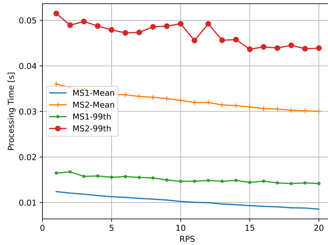
Figure 6.6: The average and the 99th percentile of the processing time for MS 1 and MS 2 from RPS 1 to RPS 20.
