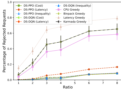
(a) Number of Rejected Requests.
