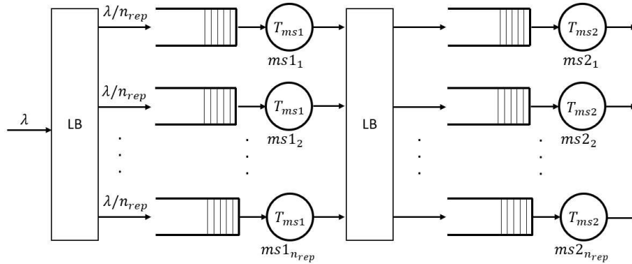
Figure 6.10: Example: a two-layered queuing system with n_{rep} replicas for both layers. In the first layer, on average, the load balancer (LB) equally distributes requests among replicas.
