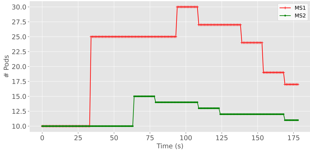
Figure 6.27: Distribution of the number of pods for each microservice during the simulation time.
