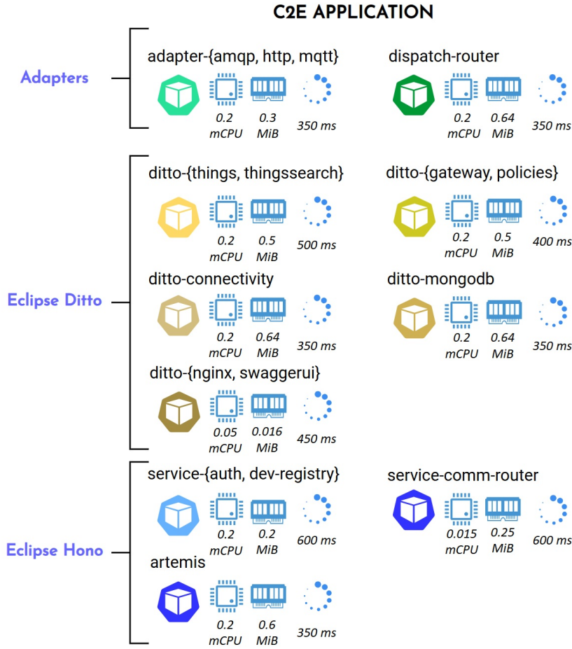
Figure 5.3: The Eclipse Cloud2Edge (C2E) architecture: processing sensor data with a DT cloud platform.
