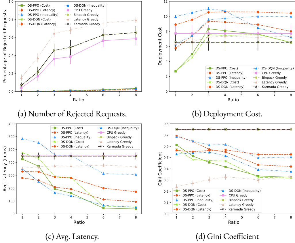
Figure 5.10: The results for the trained DS-based algorithms while varying the number of deployed replicas per request.
