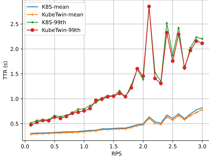
Figure 6.21: Comparison between the mean and 99th percentile response time of the real application and KT, with sd = 10 and 1 replica for each microservice.
