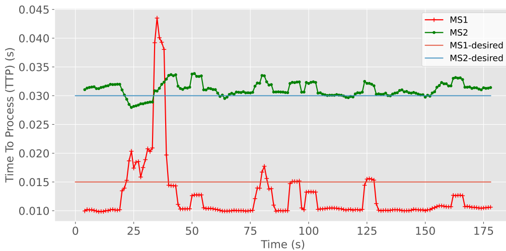
Figure 6.26: Average Time-to-Process requests per micro-service during the simulation time compared to the desired Time-to-Process.
