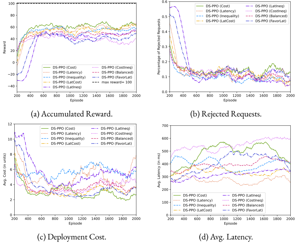
Figure 5.7: The training results for the DS-PPO agent evaluated for the multiple reward strategies.
