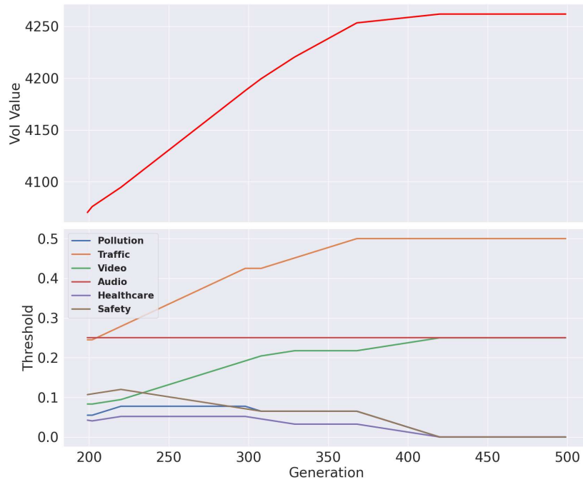
Figure 4.5: Total VoI evolution in relation to the service thresholds manipulation by GA.
