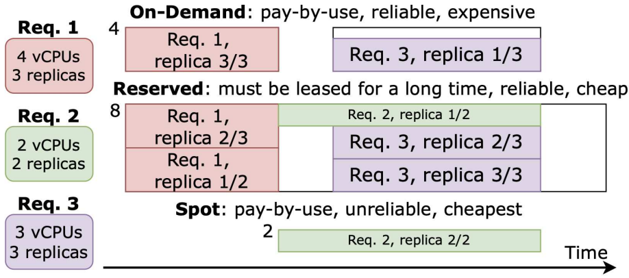
Figure 5.14: Illustrative feasible solution MO scheduling and resource allocation of K8s replicas, considering only vCPUs for ease of visualization. Replicas may be split across multiple compute instances, each with different characteristics, and must start at the same time-slot.
