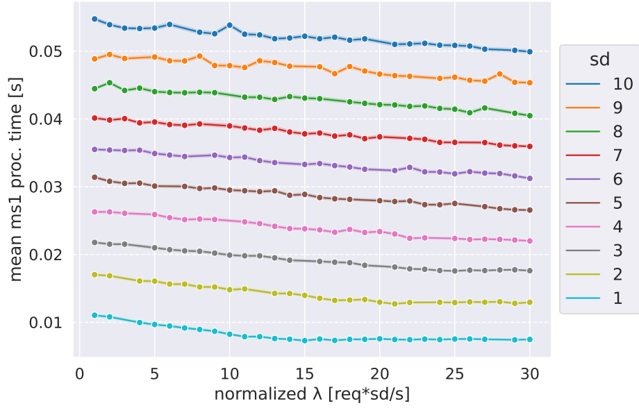
Figure 6.11: Comparison of MS1 mean proc. time, conditioned to RPS and sd factor from IX to IOX (non threaded).
