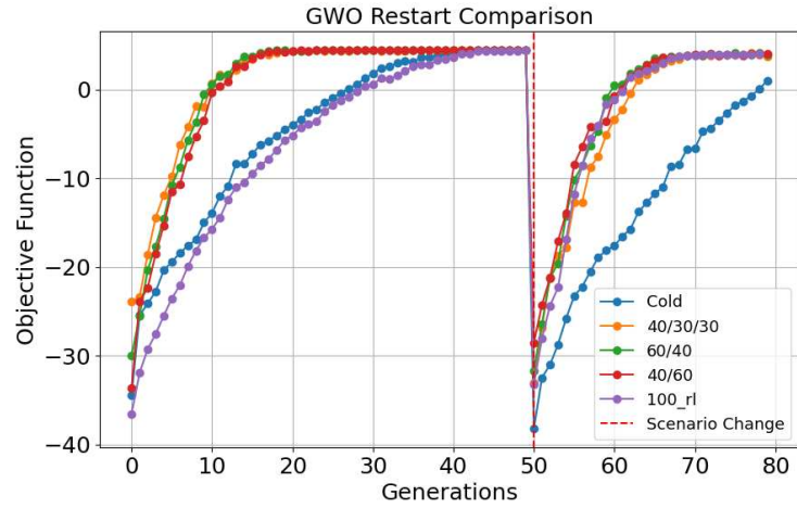
Figure 4.10: Exploitation of cold and hot restart approaches for GWO algorithm.
