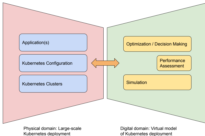
Figure 6.1: The Digital Twin concept redefined to consider Kubernetes-based software deployment.
