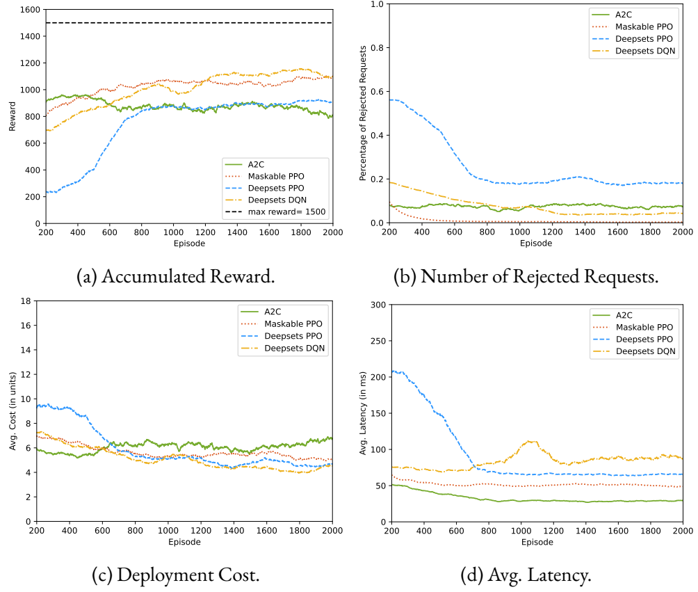
Figure 5.4: The training results for the multiple agents evaluated for the cost reward function.
