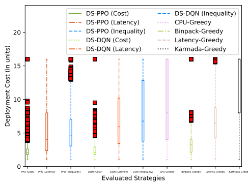
(a) Deployment Cost (in units).
