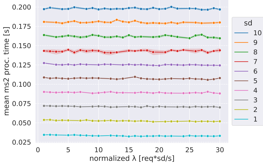
Figure 6.14: Comparison of MS2 mean proc. time, conditioned to RPS and sd factor from 1x to 10x (non threaded).
