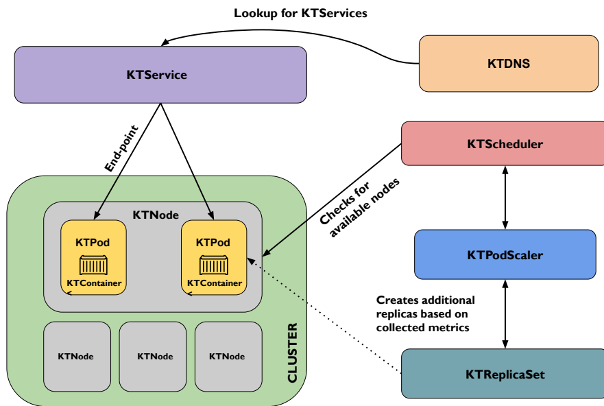
Figure 6.2: KT Architecture and interactions between components.
