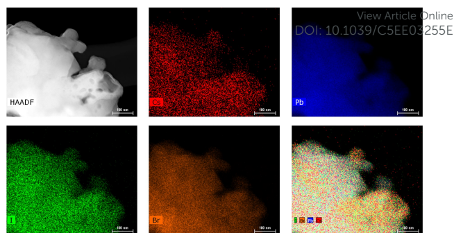
Figure 4. HAADF and TEM-EDS image of Cs 0.2 FA 0.8 PbI 2.84 Br 0.16 .
